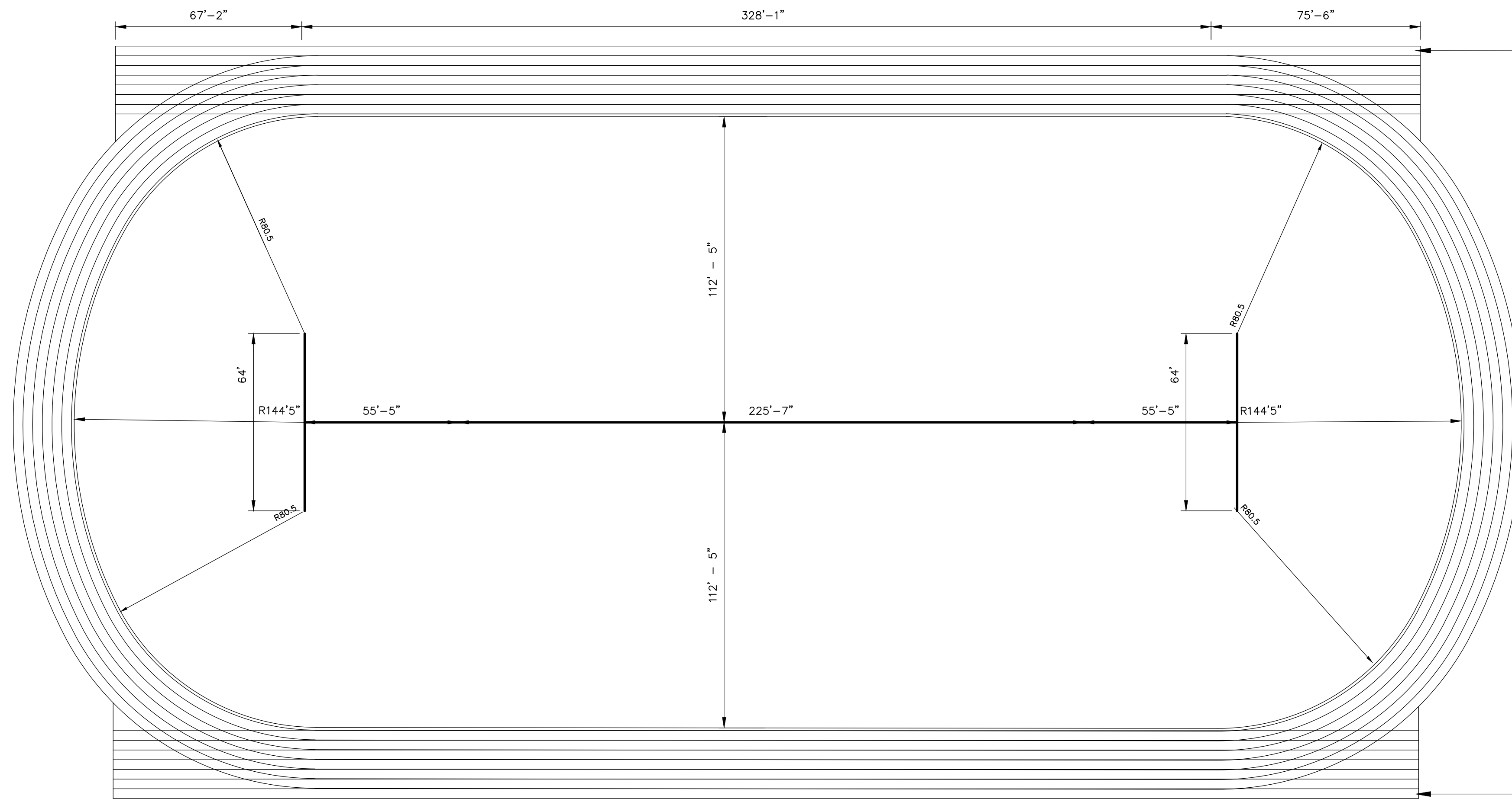
TRACK LAYOUT (BASED ON ORIGINAL TRACK DRAWINGS)
