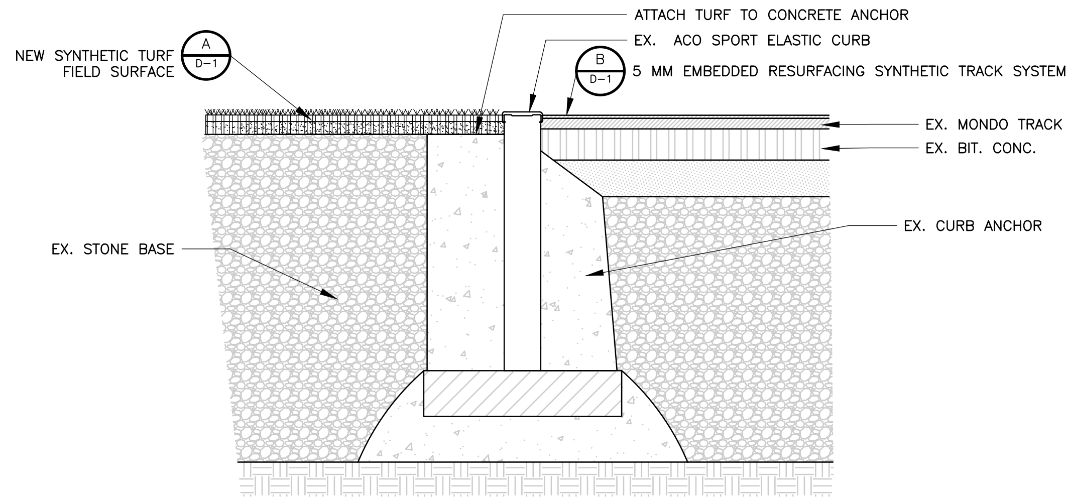
'D' AREA TURF AT EX. CURB DETAIL C NTS D-1
