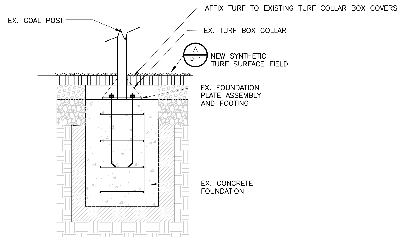
TURF AT EX. GOAL POST FOOTING DETAIL D NTS D-1
