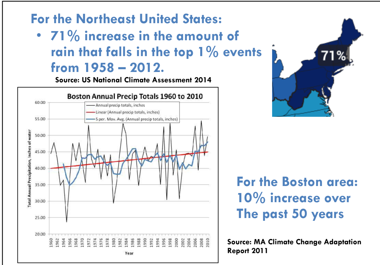
Figure 6. Observed Precipitation Change
