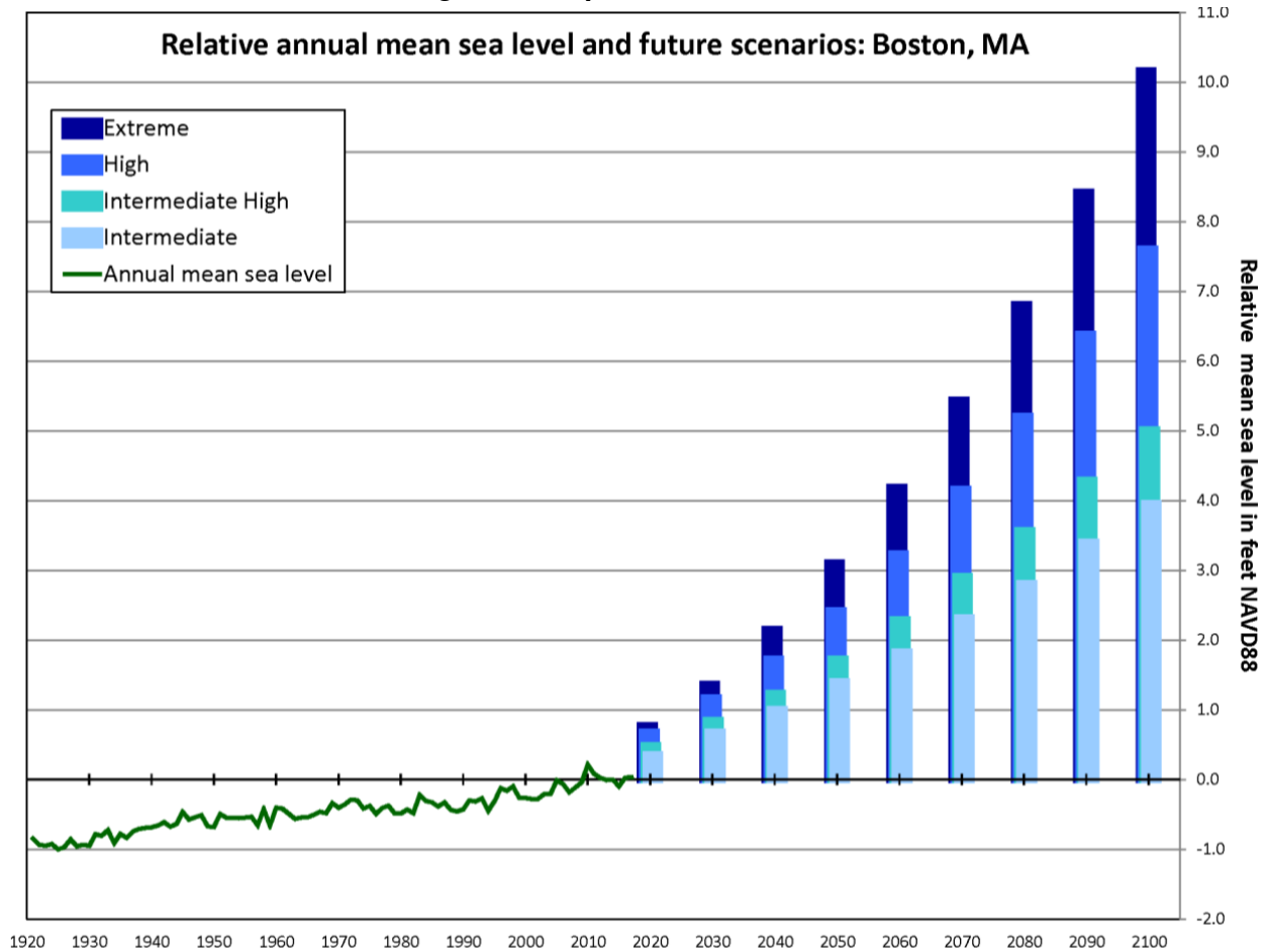
Figure 5. Projected Sea Level Rise
