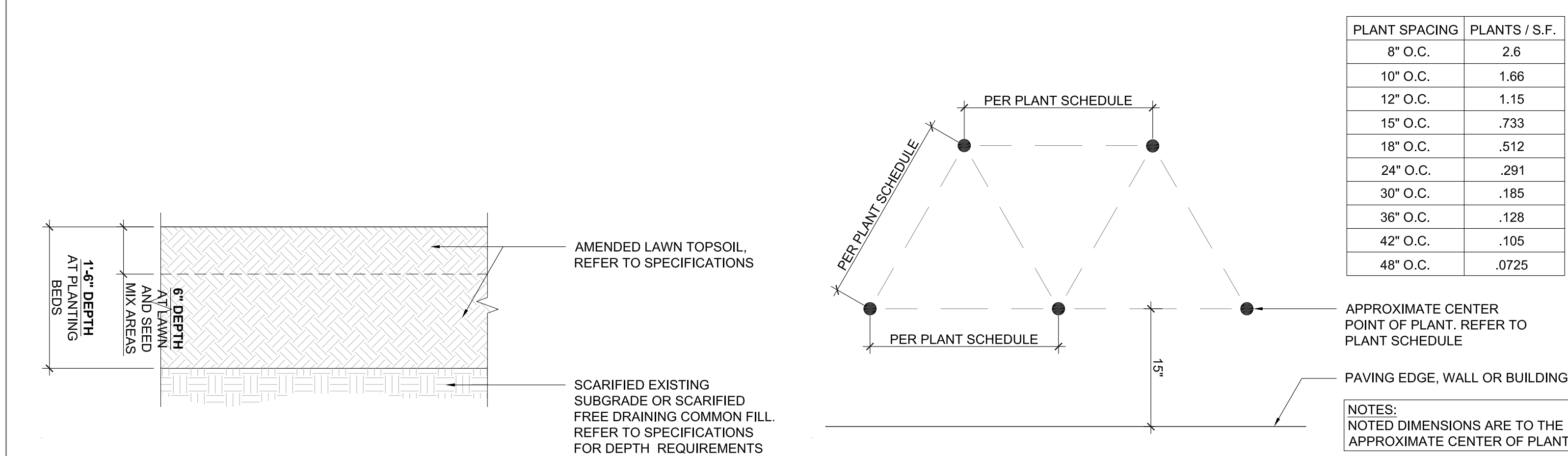
4 SOIL PREPARATION 1.4.02 SCALE: 1" = 1'-0"
