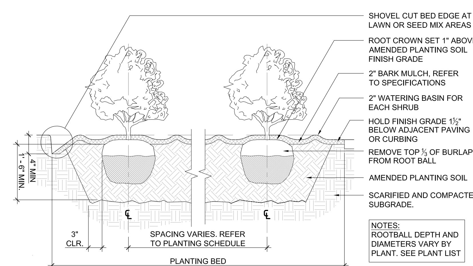
2 SHRUB / GROUNDCOVER / PERENNIAL PLANTING 1.4.02 SCALE: NTS
