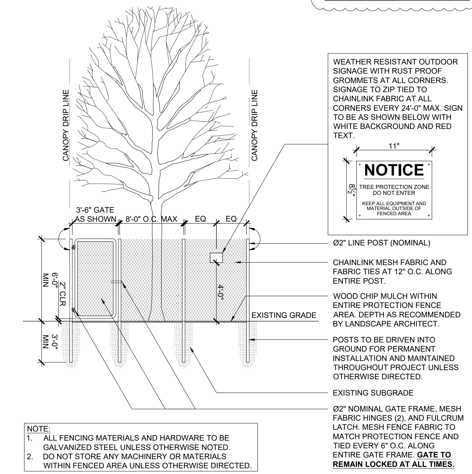
1 TREE PROTECTION FENCING 1.4.03 SCALE: 1/2" = 1'-0"
