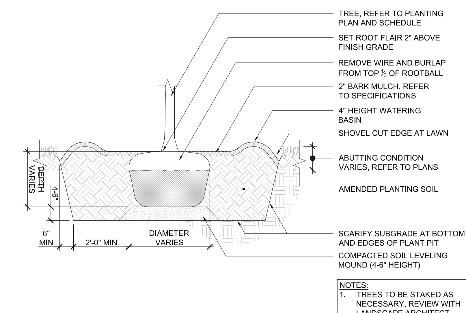
1 TREE PLANTING 1.4.02 SCALE: 1/2" = 1'-0"
