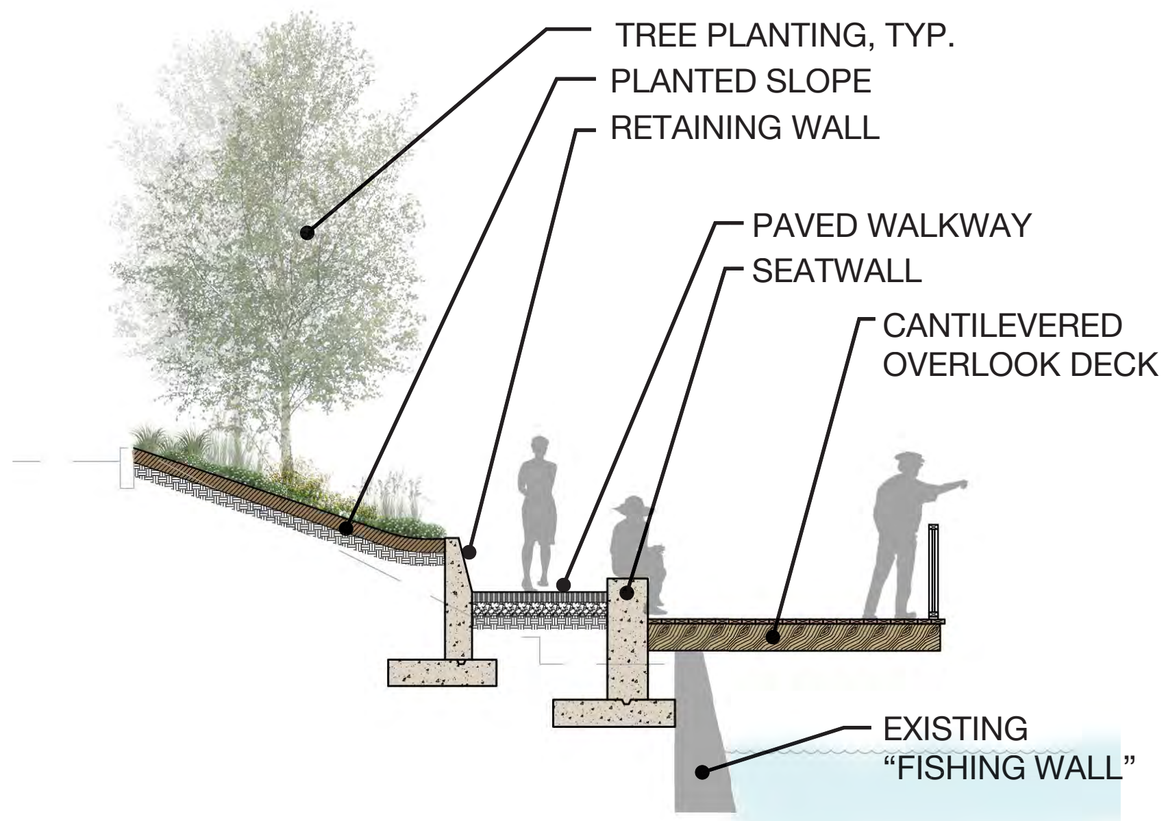
SECTION AT FISHING WALL
