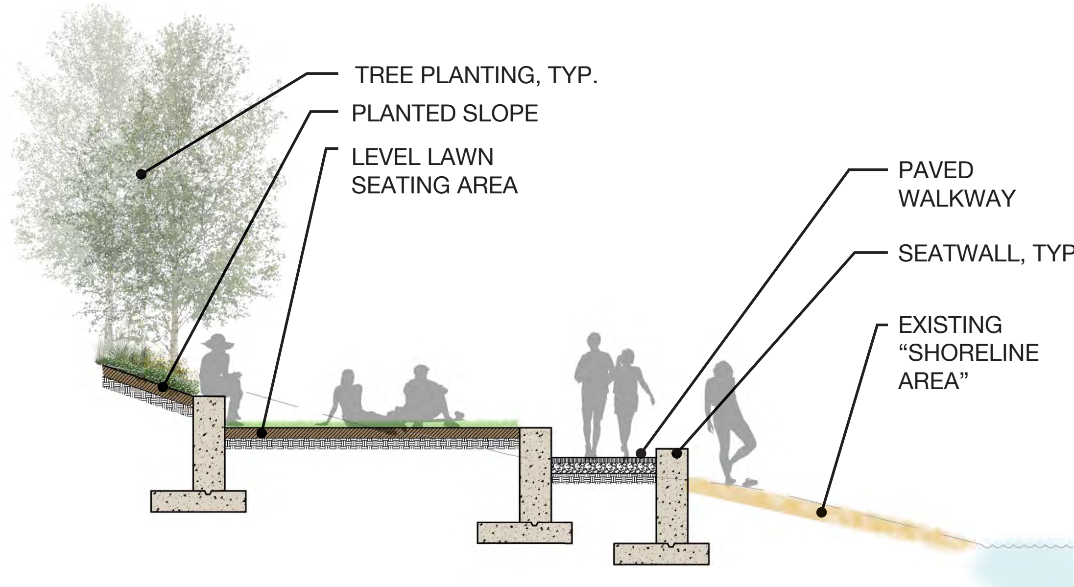
SECTION AT SHORELINE AREA
