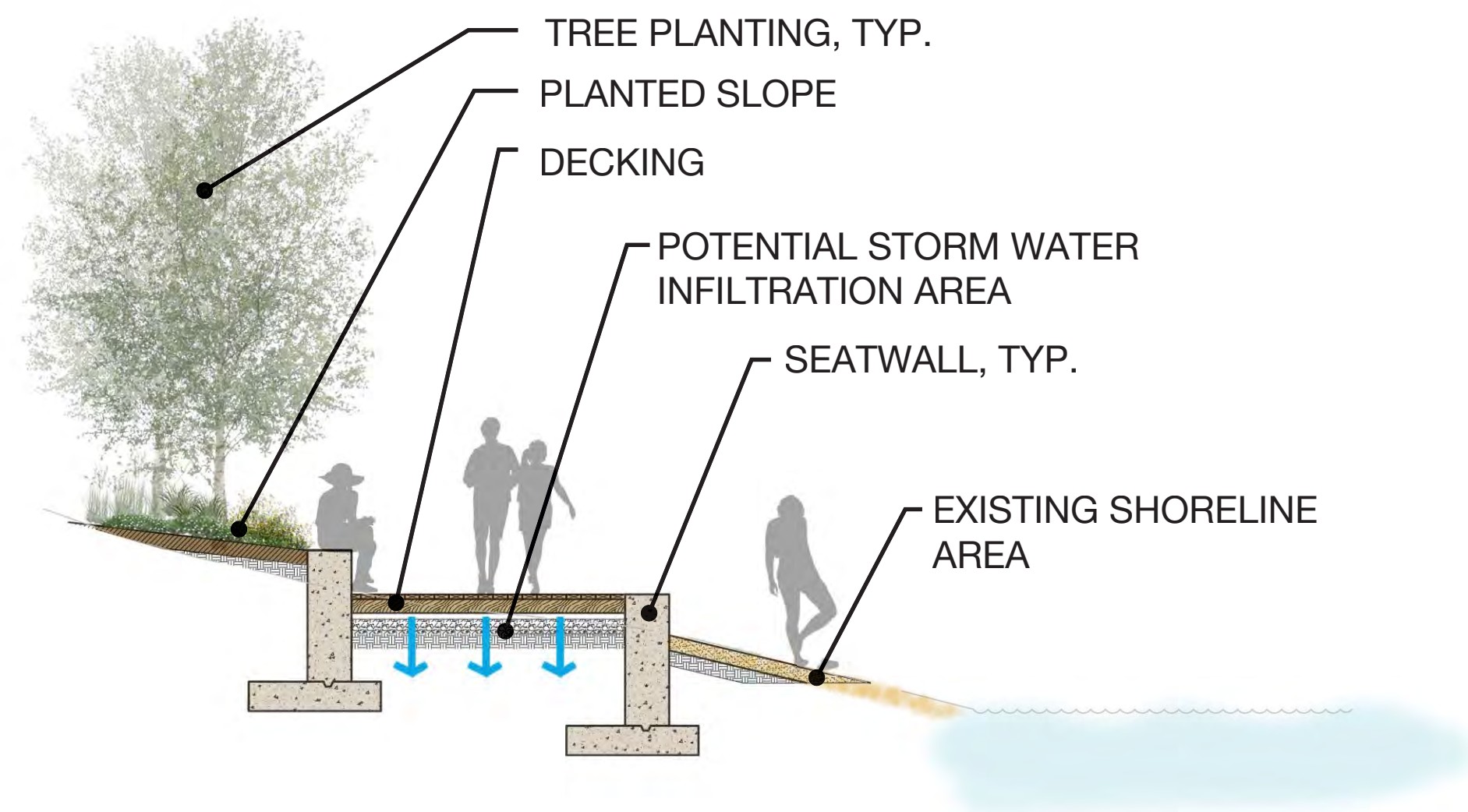
SECTION AT SHORELINE AREA
