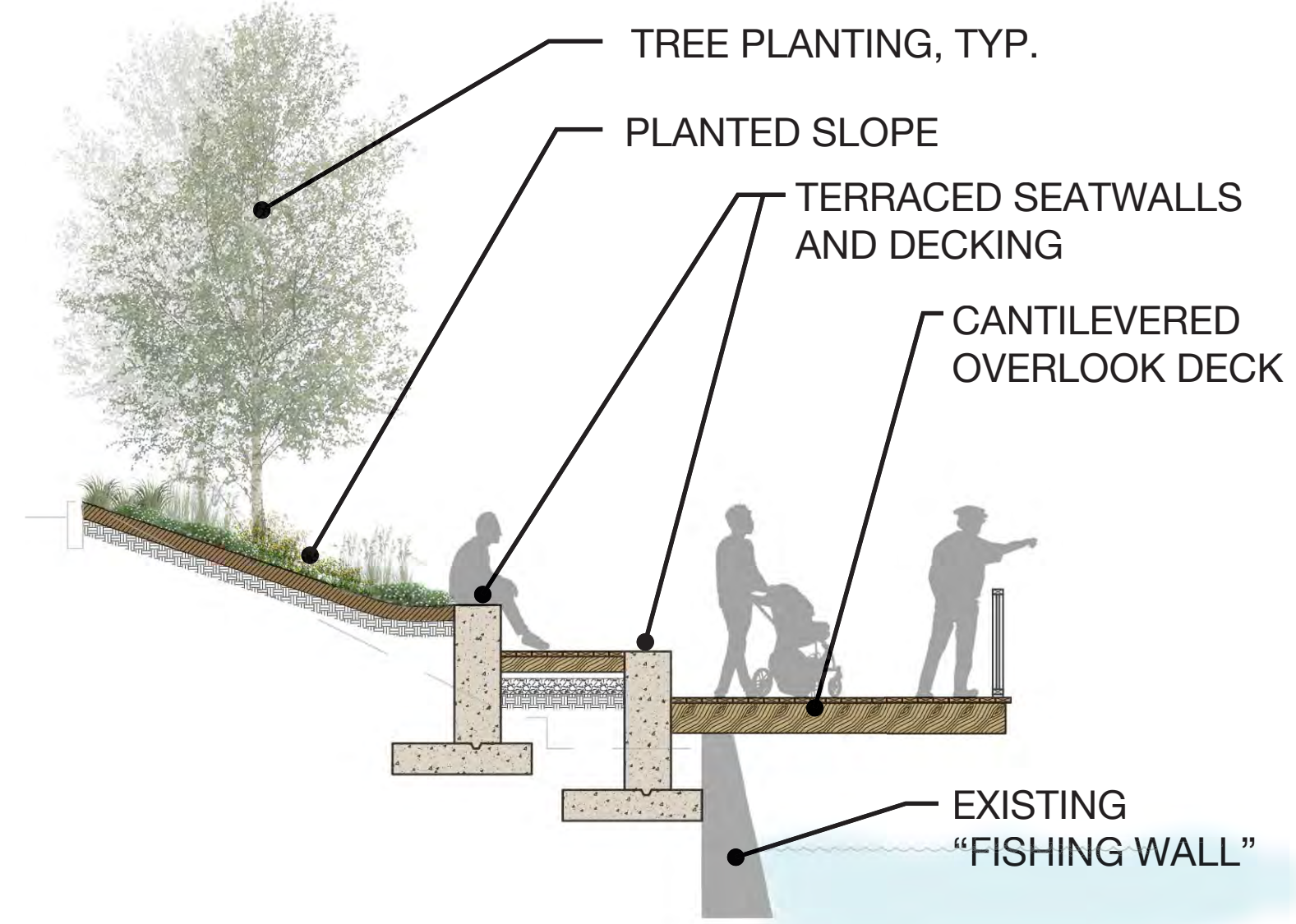
SECTION AT FISHING WALL
