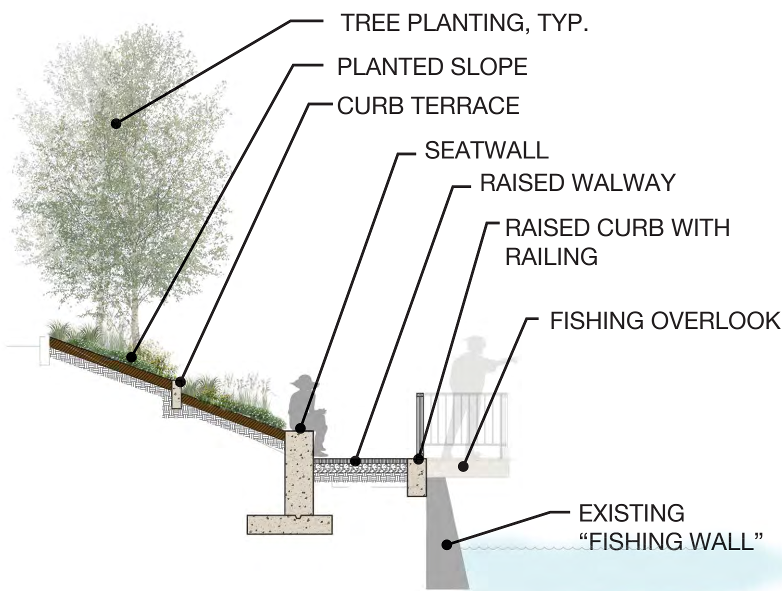
SECTION AT FISHING WALL
