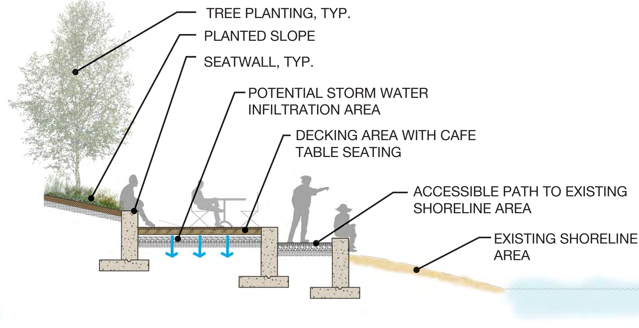
SECTION AT SHORELINE AREA
