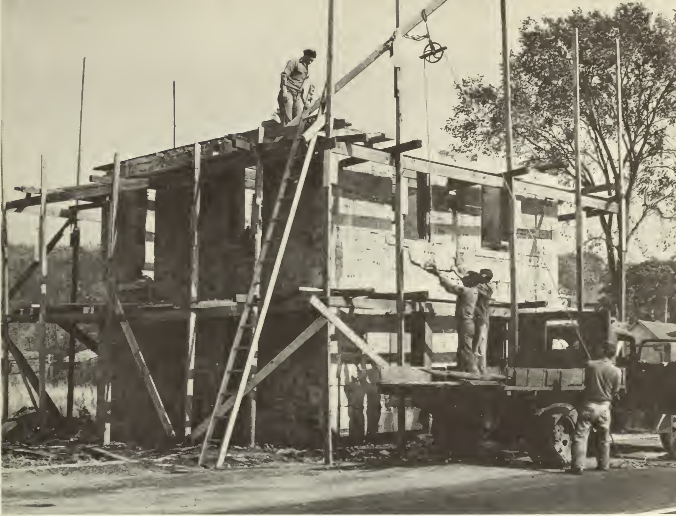
Figure 22: Disassembly of a stone masonry building in Mystic, Connecticut
