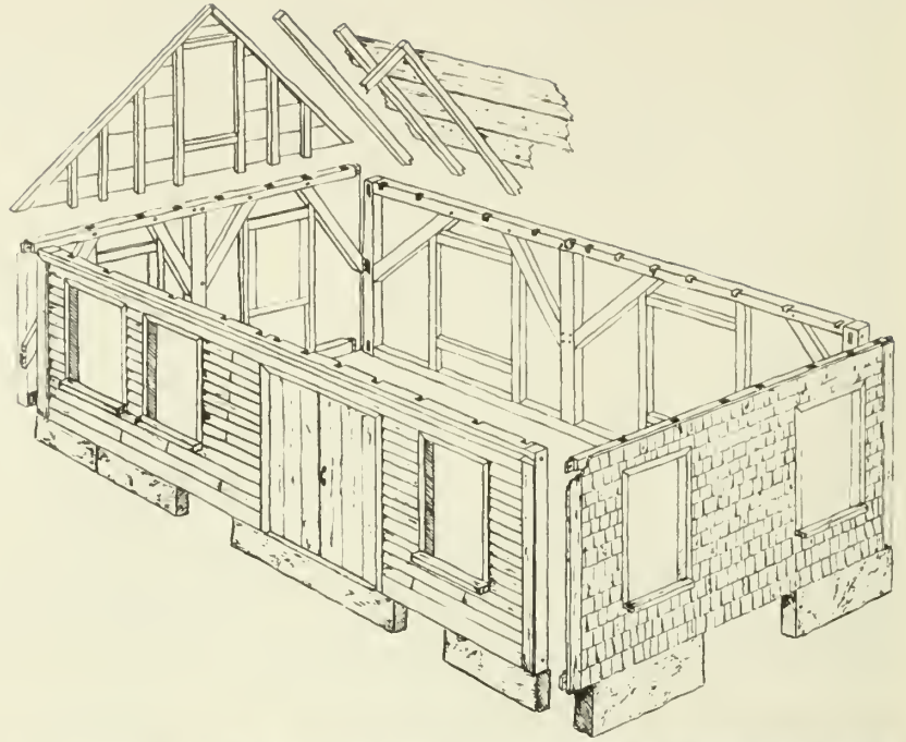
Figure 23: A schematic drawing of the circa 1830 Hapgood Carding Mill in South Waterford, Maine, details a method of partial disassembly. Roof components must be marked and disassembled in their entirety prior to separating the remainder of the structure into six major elements. [Sketch by John O. Curtis, Old Sturbridge Village]
