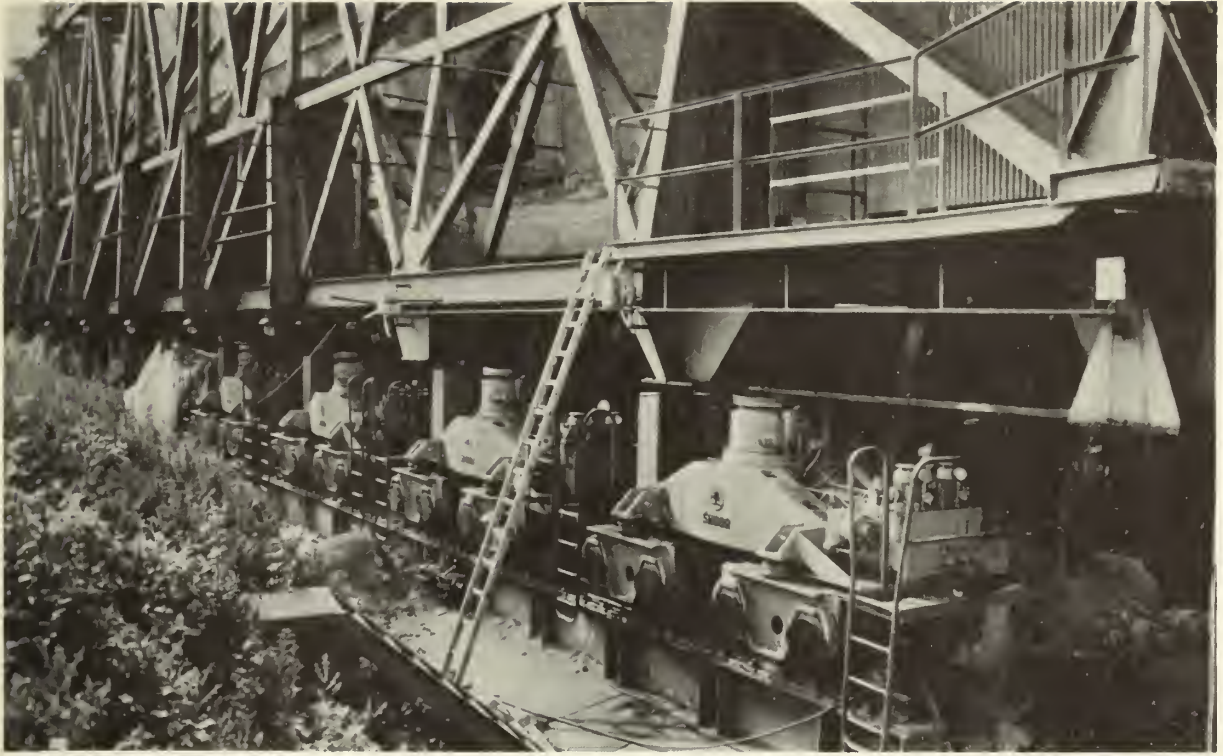
Figures 13–14: The weight of the church and its steel supportive superstructure, together totaling 10,560 tons, was raised to allow the emplacement of more than 50 trolleys (figure 13) which carried the church over four sets of train tracks to its new site (figure 14). [Figure 13 from a slide by Jack E. Boucher, 1975. Figure 14 photograph by W. Preiss, Dresden, 1975, courtesy of Jack E. Boucher]
