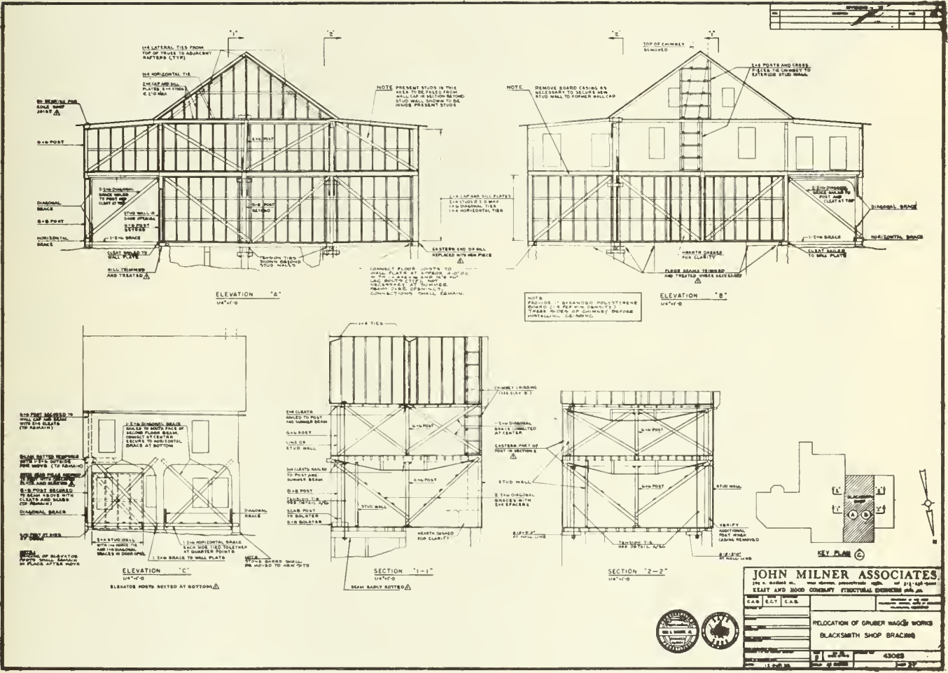
Figure 37: Working drawing, "Blacksmith Shop Bracing."
