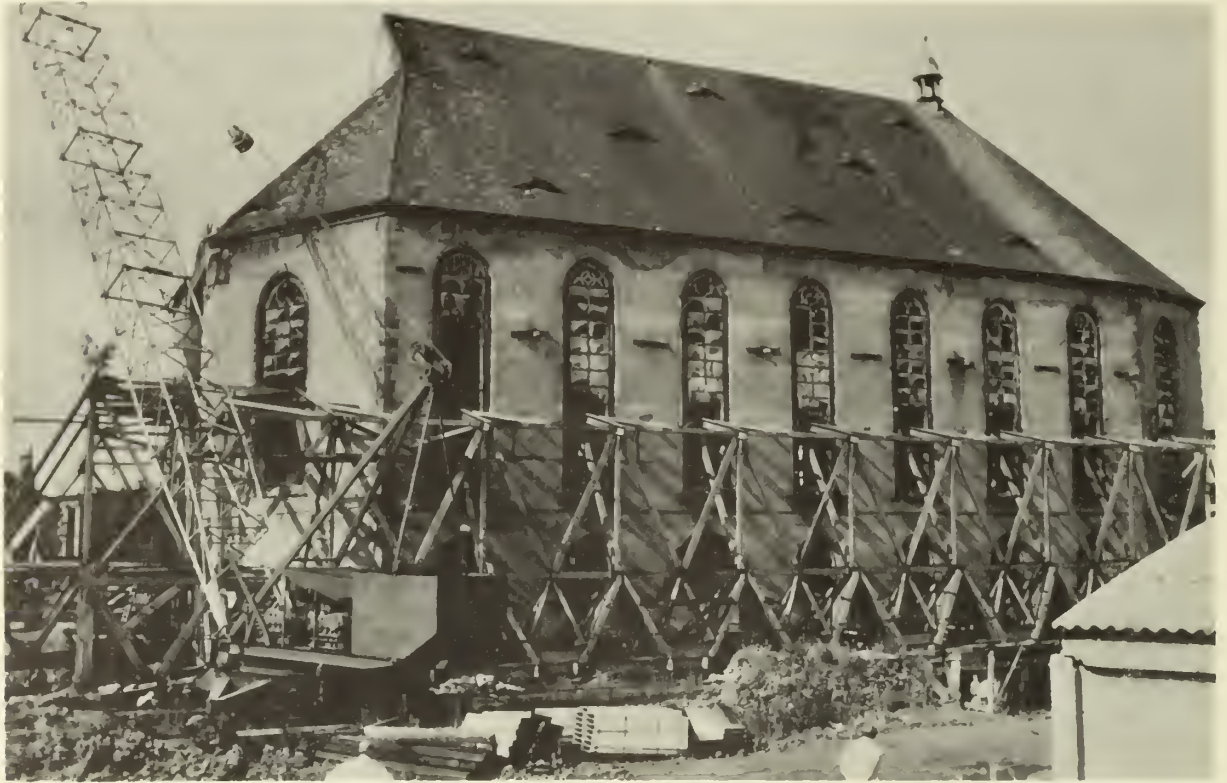
Figure 12: The first step in the moving process was to remove the later addition of a tower (not seen here). Then a steel girdle was constructed, approximately 197 feet long by 97 feet wide by 103 feet high, to encircle the structure. [Photograph from a slide by Jack E. Boucher, 1975]
