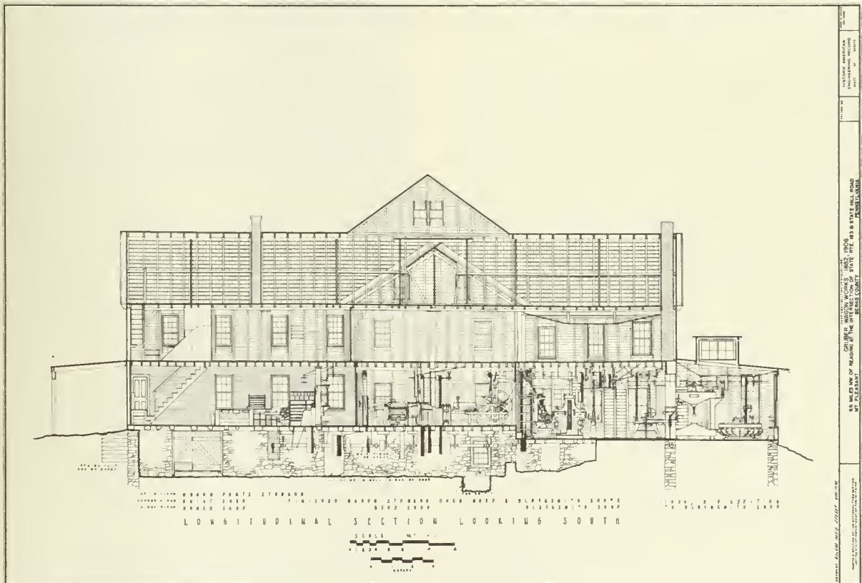
Figure 34: Measured drawing
