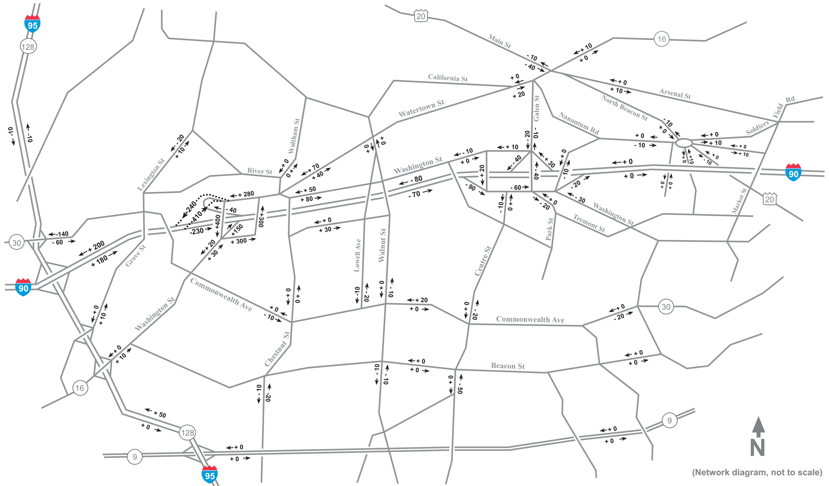
Figure 11: Alternative 3 - Projected 2030 AM Peak-Hour Traffic-Volume Changes from No-Build
