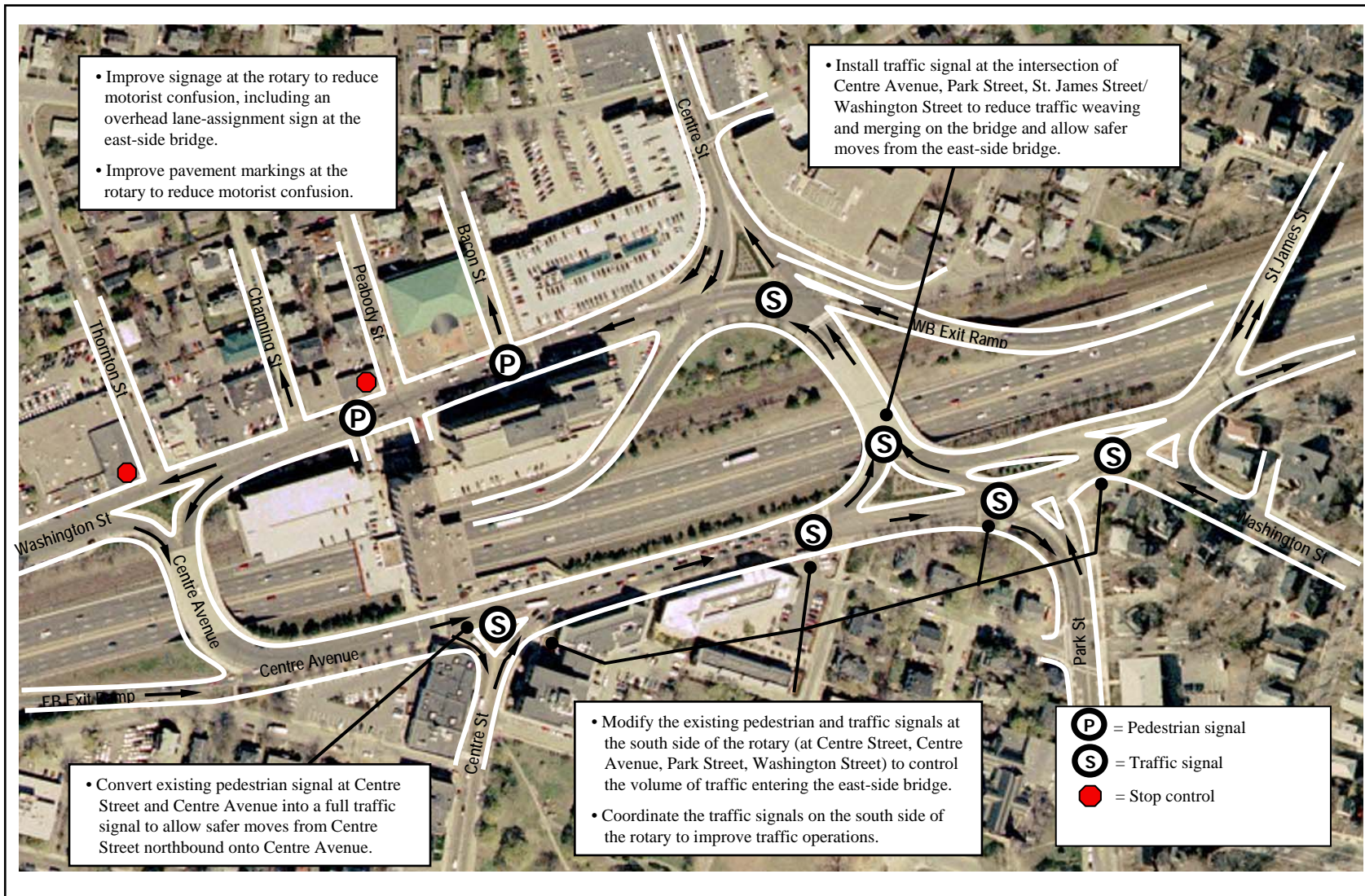
Figure E-1: Improvements Tested in Alternative 5
