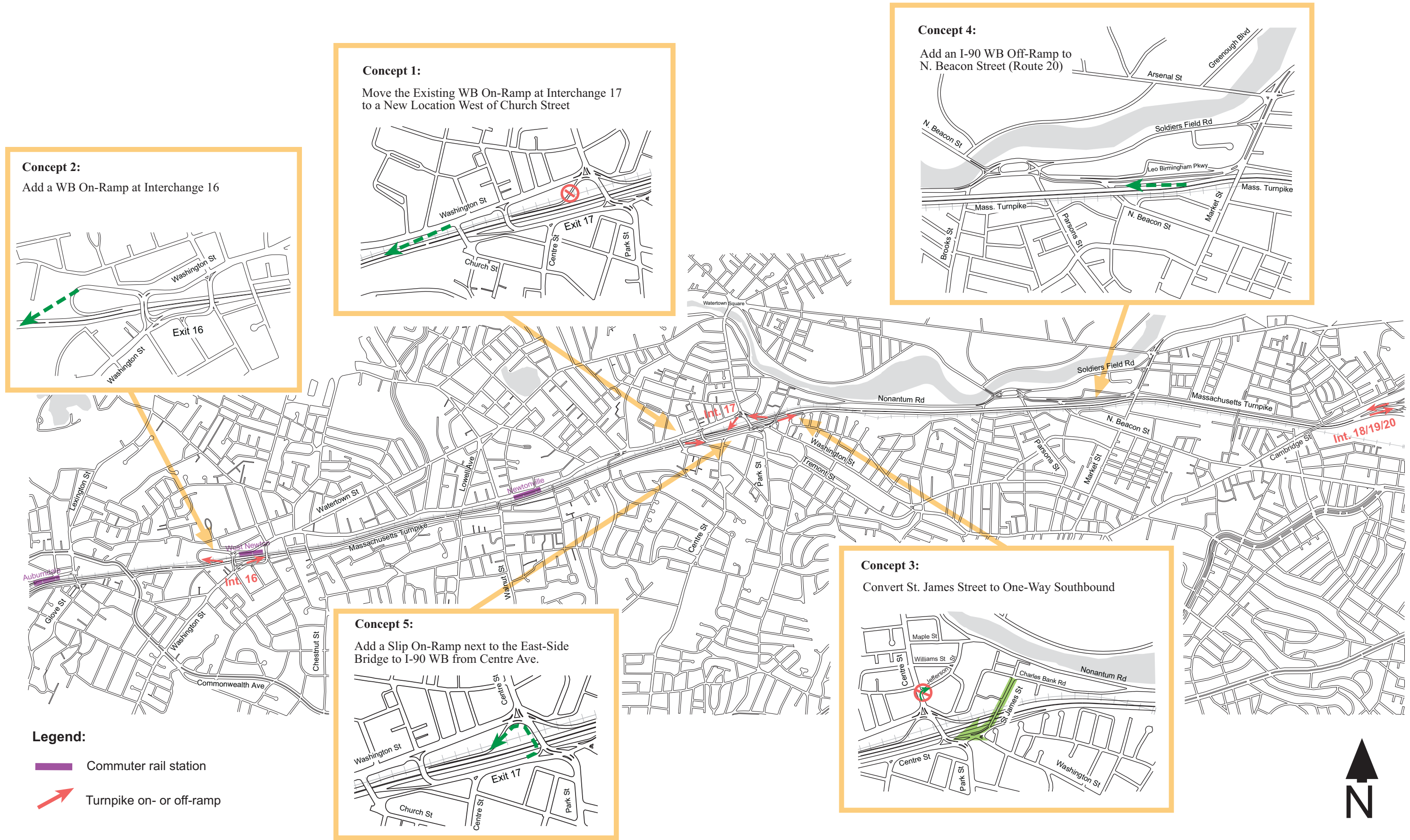
Figure 2: Improvement Concepts 1 to 5
