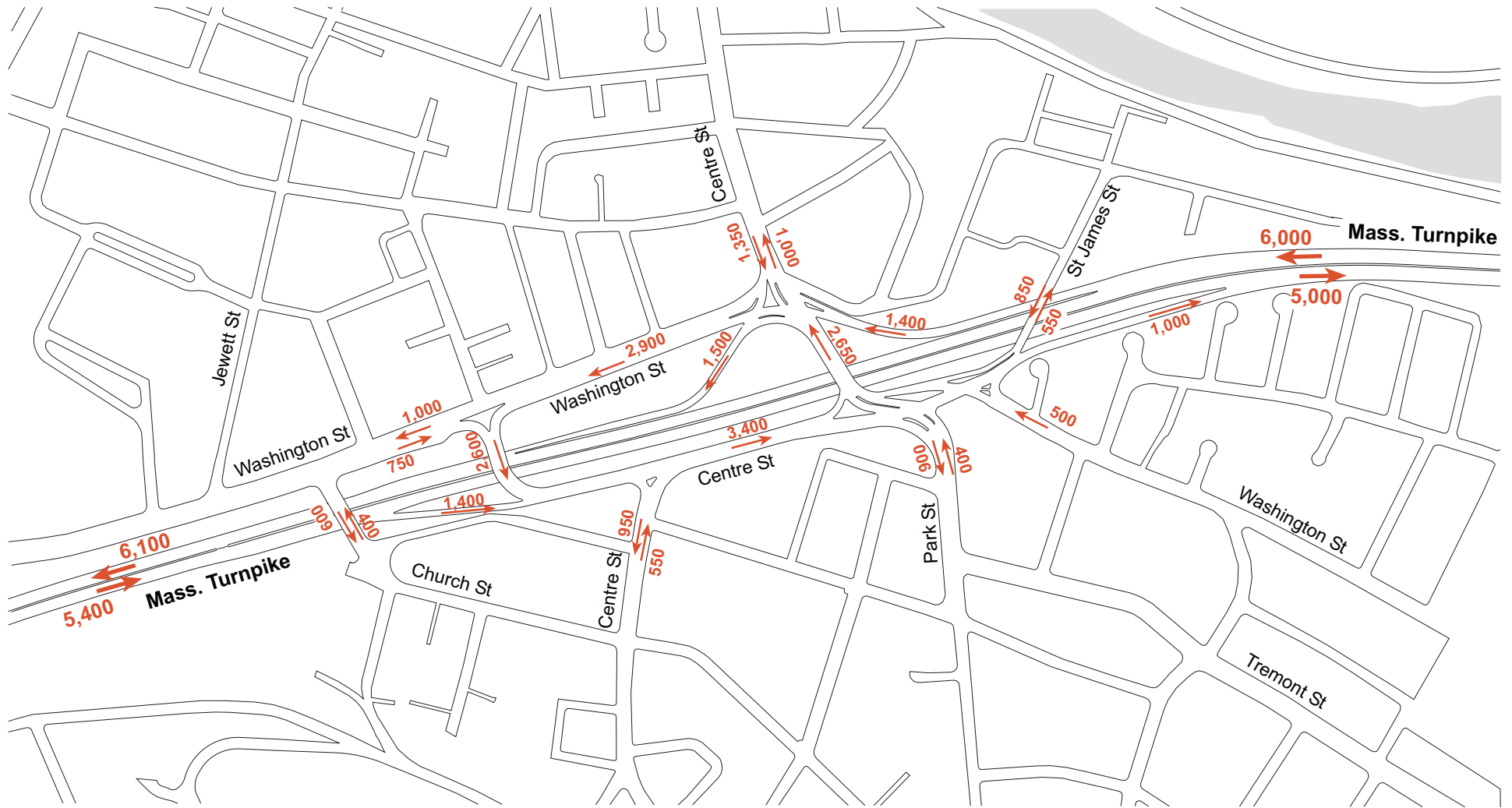
Estimated Existing (2006) Weekday PM Peak-Hour (5:00-6:00 PM) Traffic Volumes
