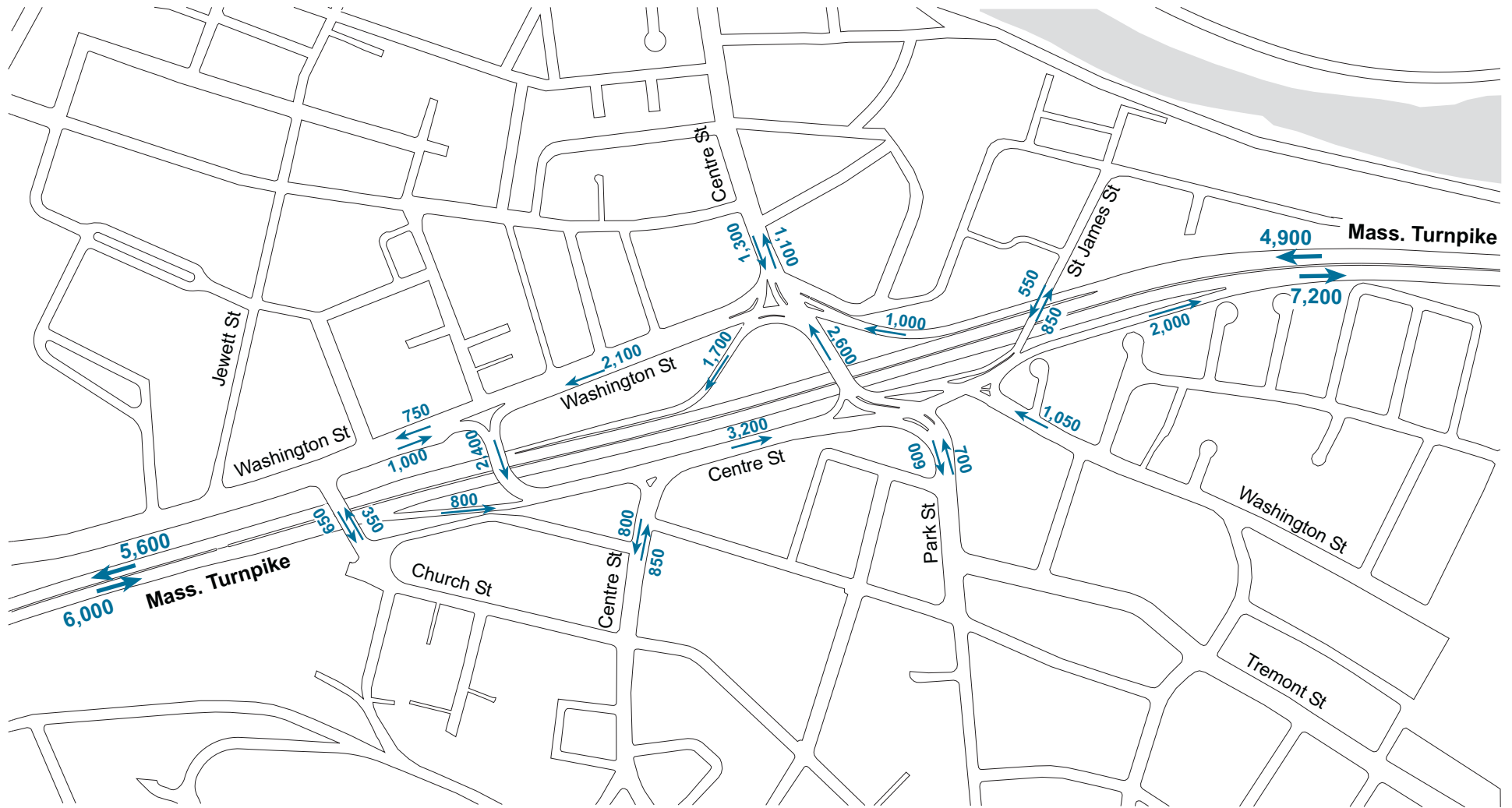
Estimated Existing (2006) Weekday AM Peak-Hour (8:00-9:00 AM) Traffic Volumes
