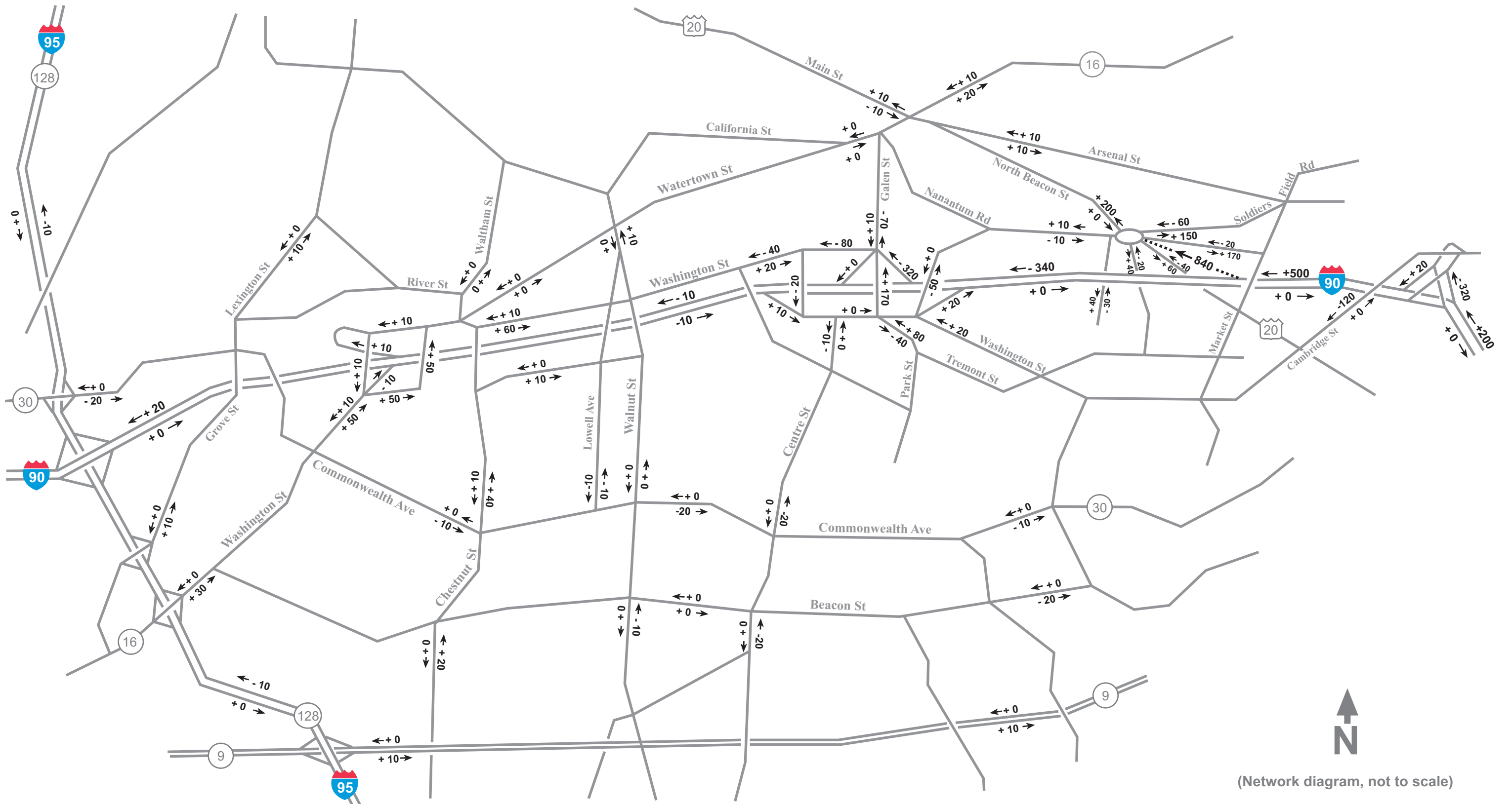
Figure 9: Alternative 2 - Projected 2030 AM Peak-Hour Traffic-Volume Changes from No-Build
