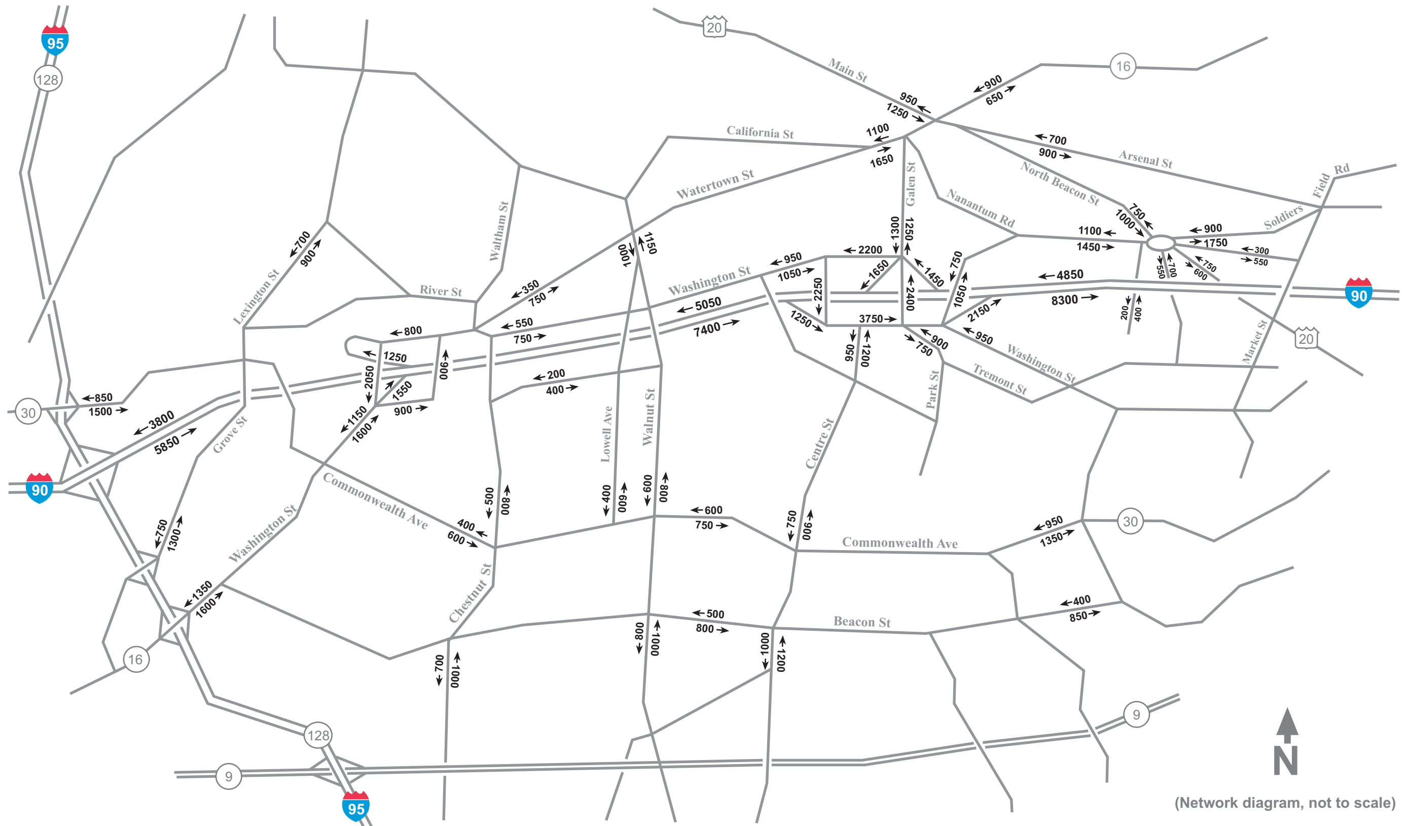
Figure 7: Alternative 1 (No-Build) - Projected 2030 AM Peak-Hour Traffic Volumes
