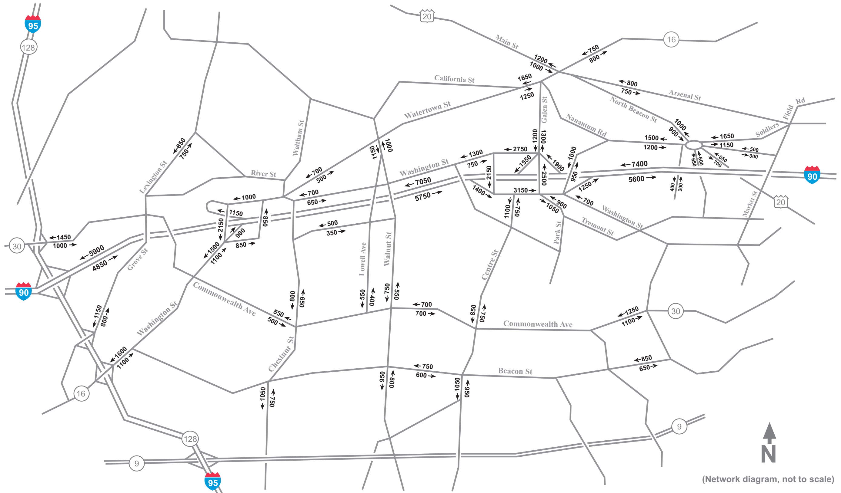
Figure 8: Alternative 1 (No-Build) - Projected 2030 PM Peak-Hour Traffic Volumes
