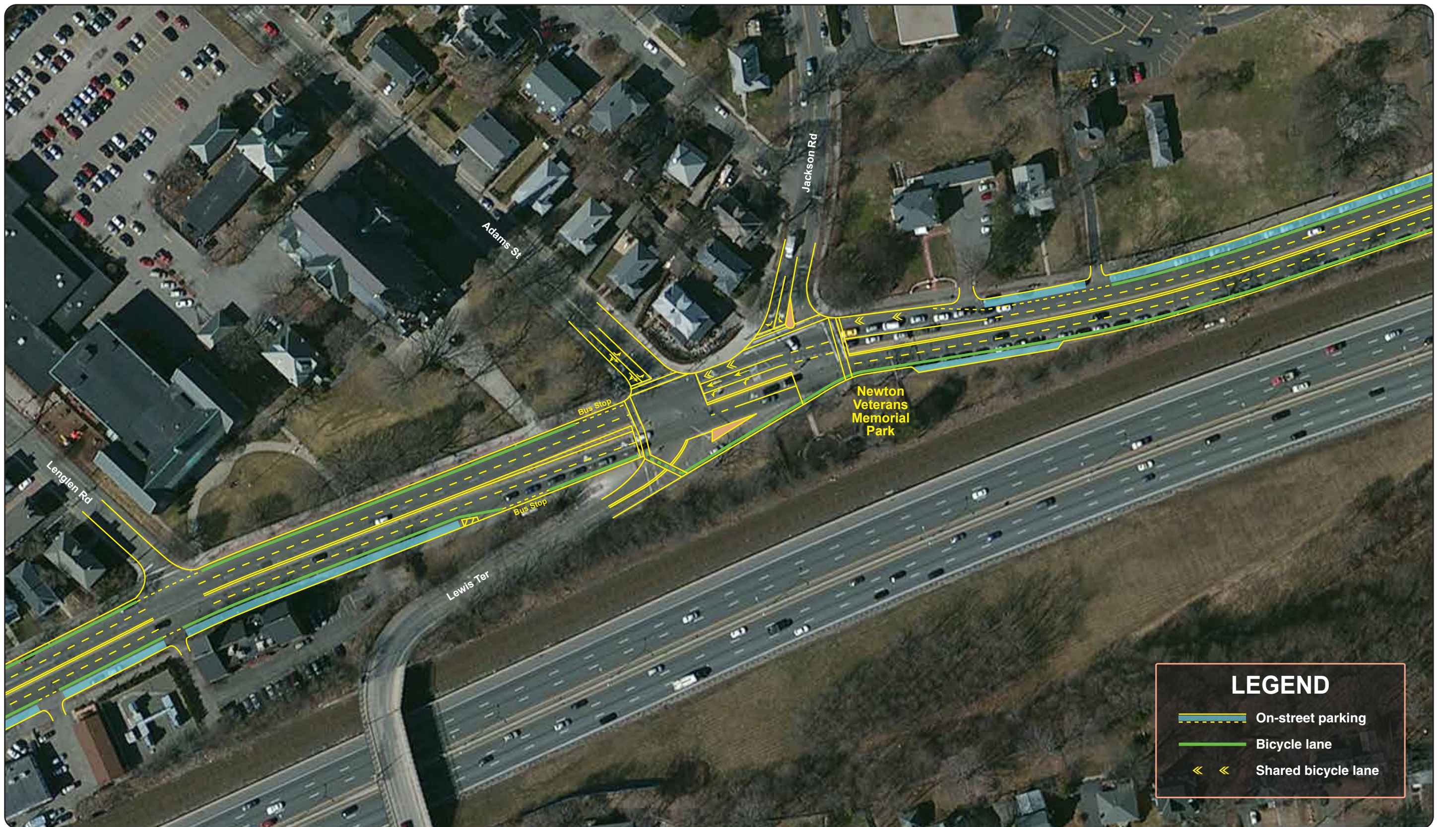
FIGURE 7-6 Conceptual Plan of Proposed Long-Term Improvements (Section 6) Washington Street, Newton
