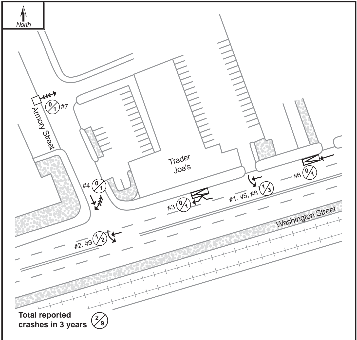
FIGURE F-2 Intersection Collision Diagram, Newton Police Reports 1/1/2011–2/28/2014 Washington Street @ Armory Street
