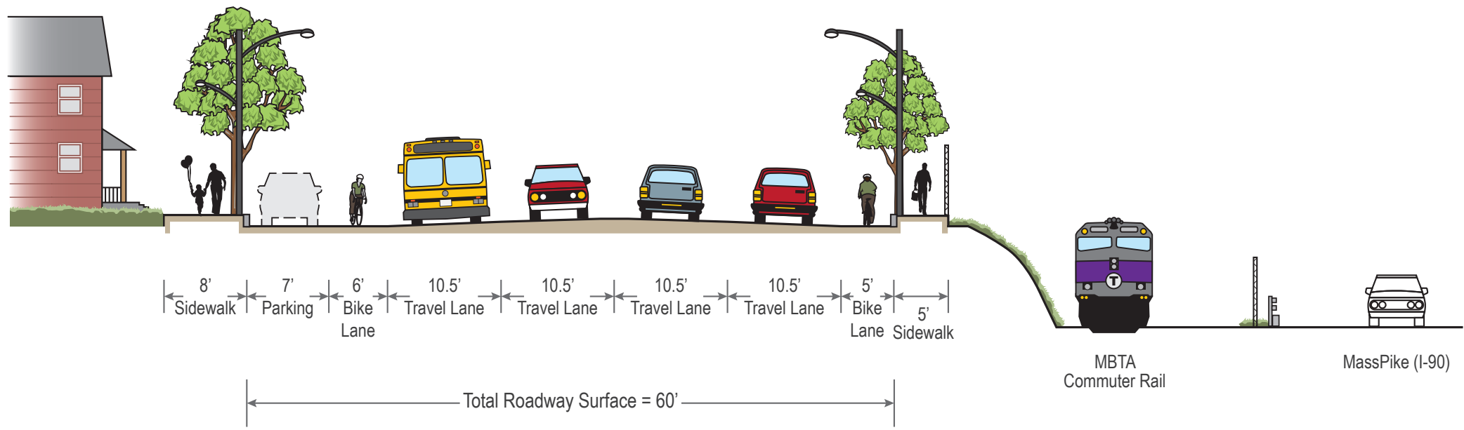
Proposed Four-Lane Cross-Section
