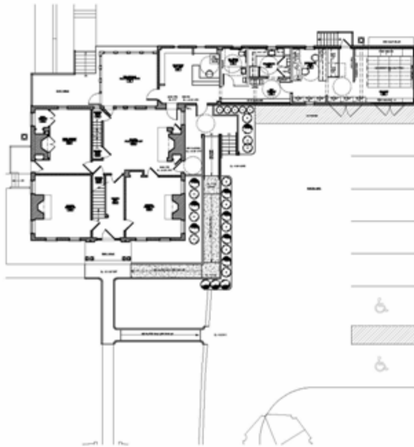
Proposed Site Plan SCALE: 1/16" = 1'-0"
