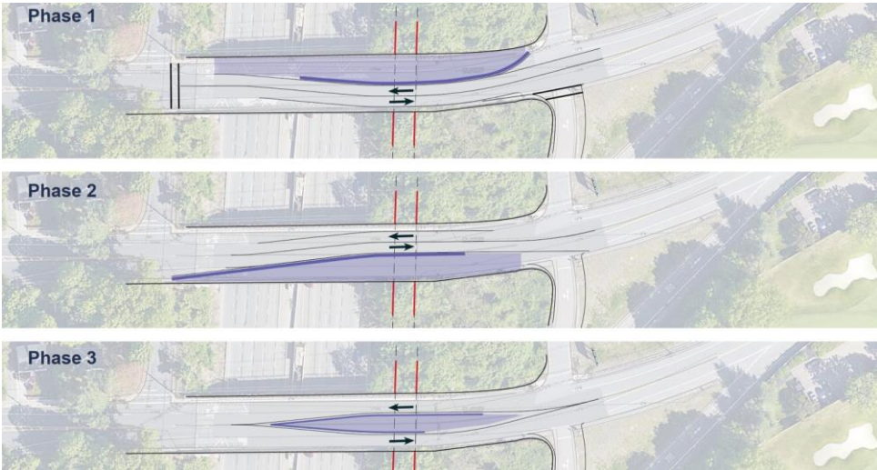
Figure 9 – Grove Street Bridge Traffic Maintenance
