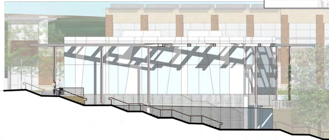
WEST ELEVATION SPECIAL PERMIT
