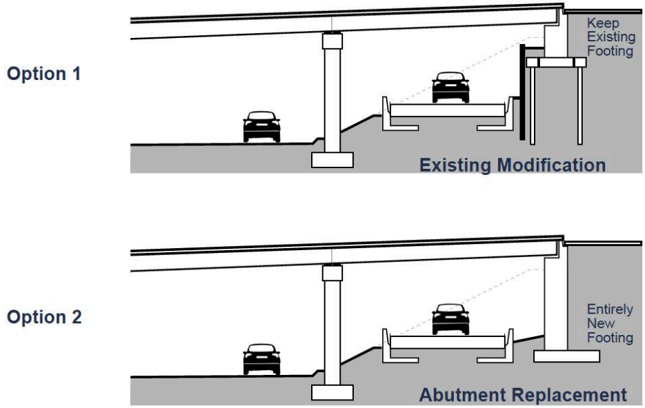
Figure 8 – Grove Street Bridge Modification Options
