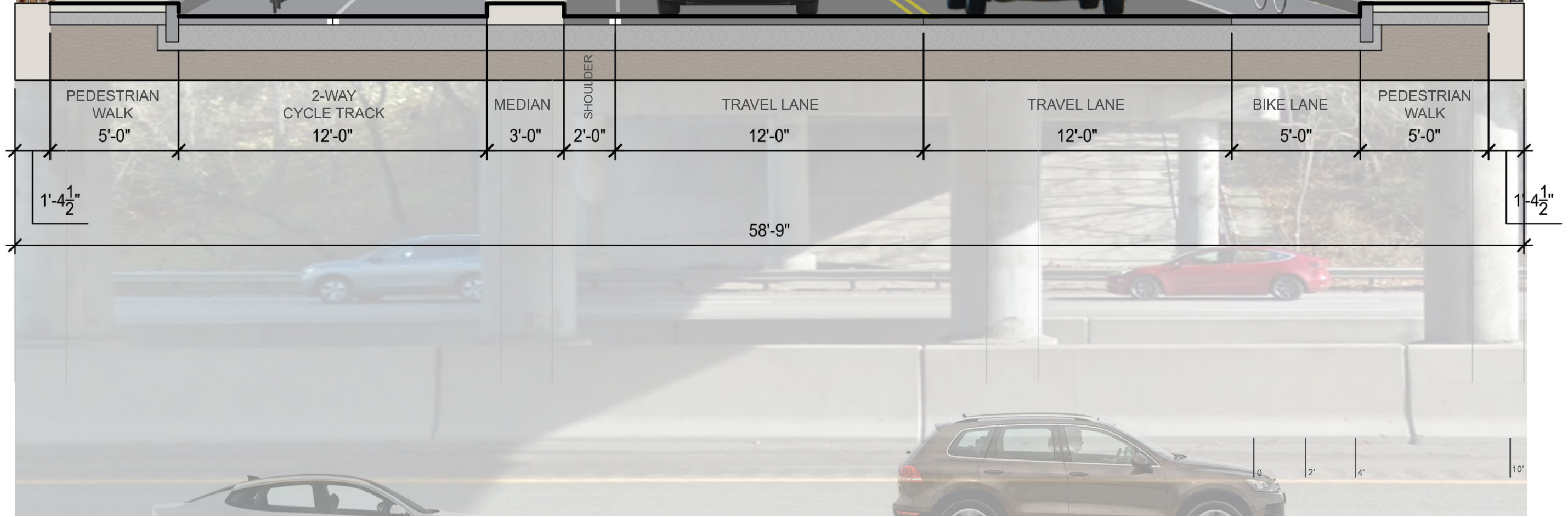
Grove Street Section - 95 Overpass (Looking Northeast)
