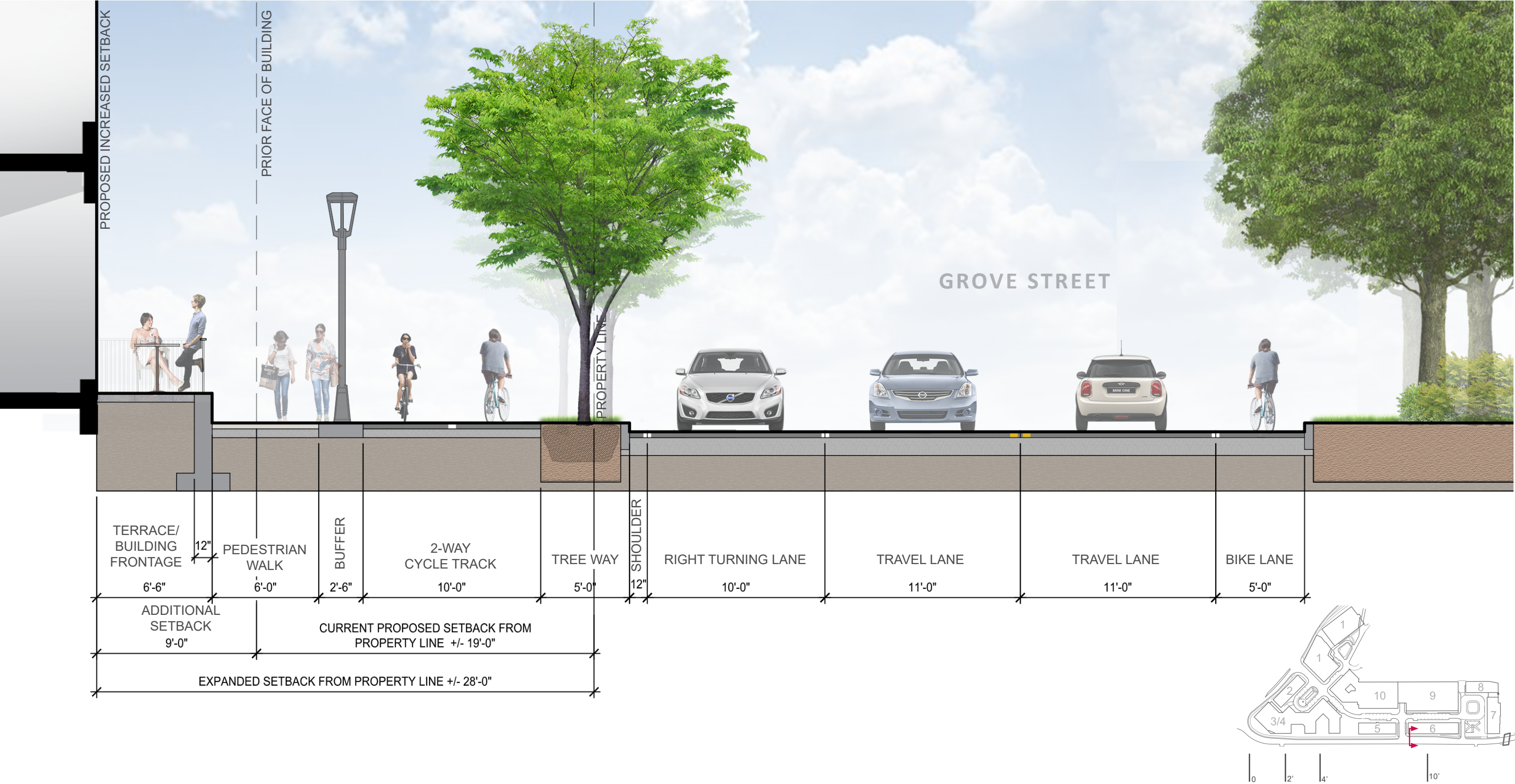
Grove Street Section - Building 6 Proposed Condition
