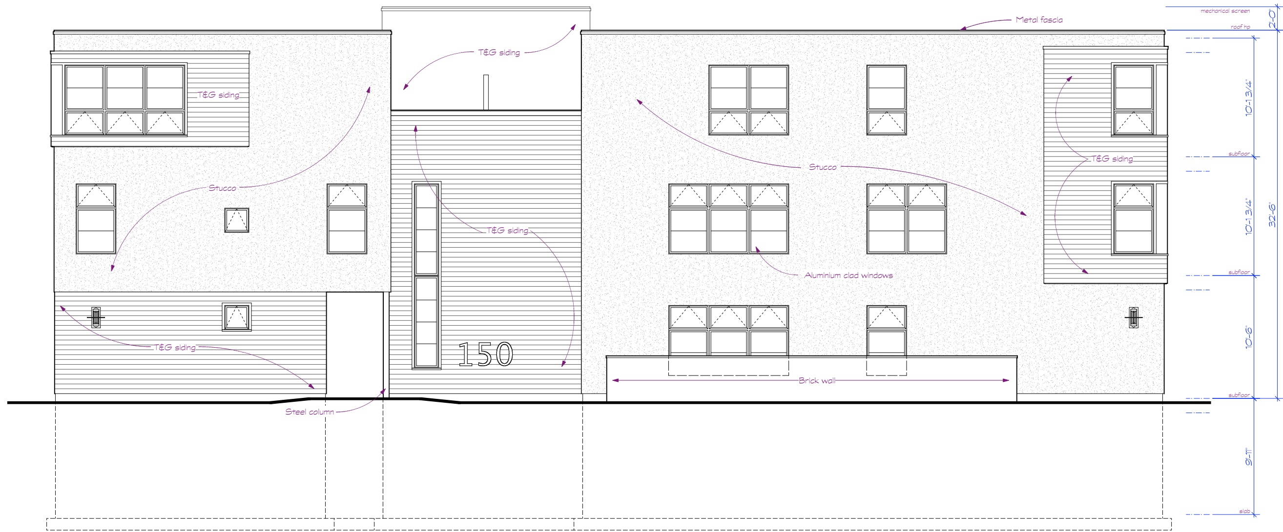
ADAMS STREET ELEVATION ① SCALE: 1/8" = 1'-0"
