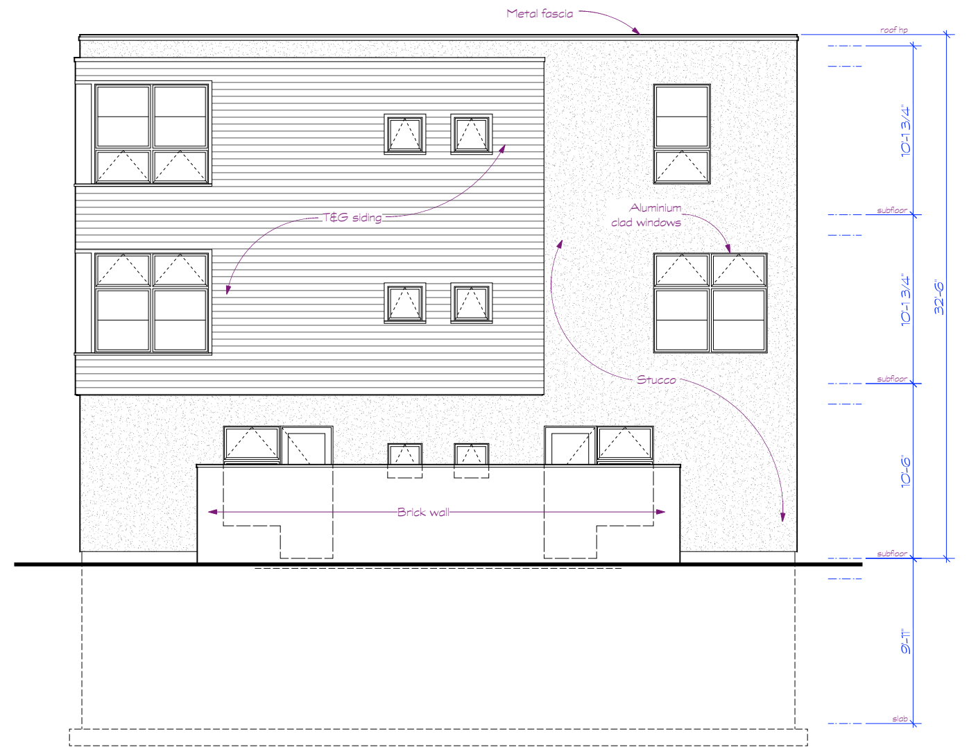
COTTAGE COURT ELEVATION 2 SCALE: 1/8" = 1'-0"
