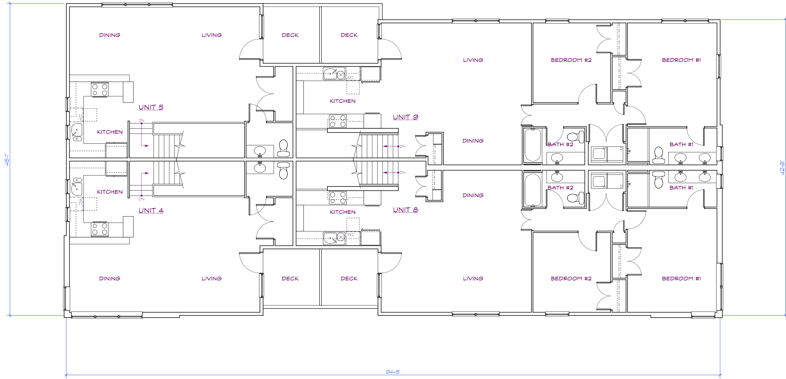
THIRD FLOOR PLAN 3 SCALE: 1/8" = 1'-0"
