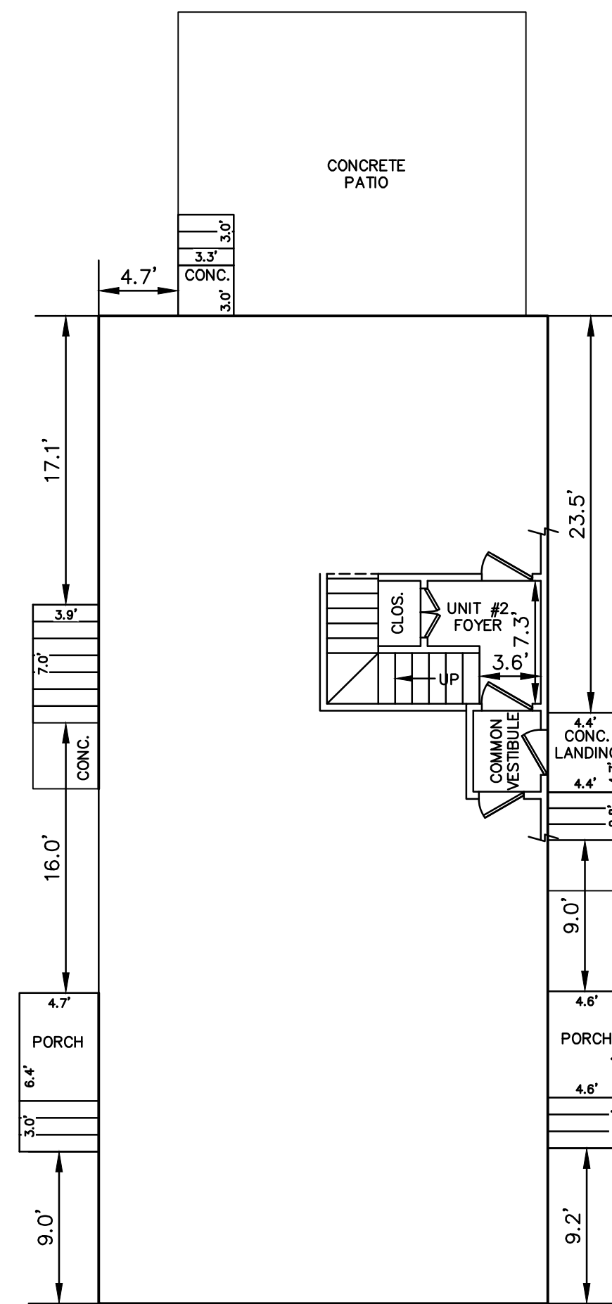
FIRST FLOOR UNIT #2 AREA=113.2 s.f.
