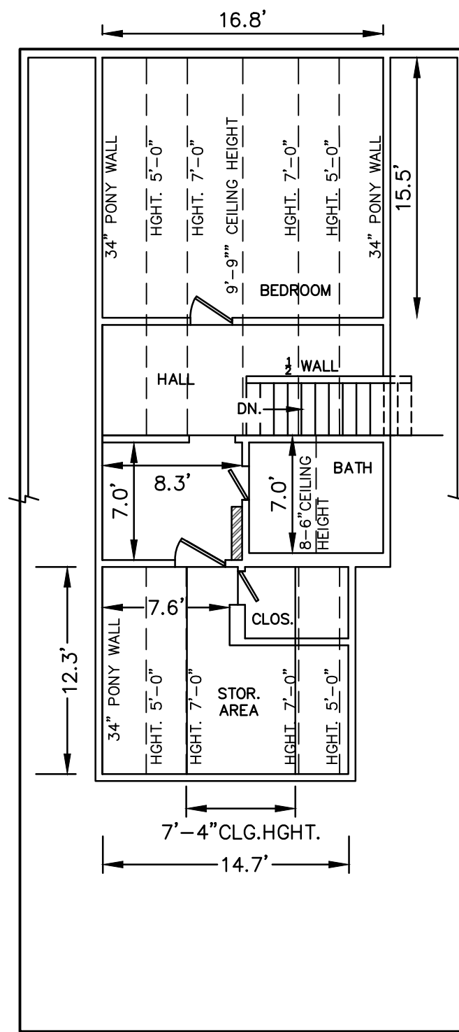
THIRD FLOOR UNIT #2 AREA=490.9 s.f.
