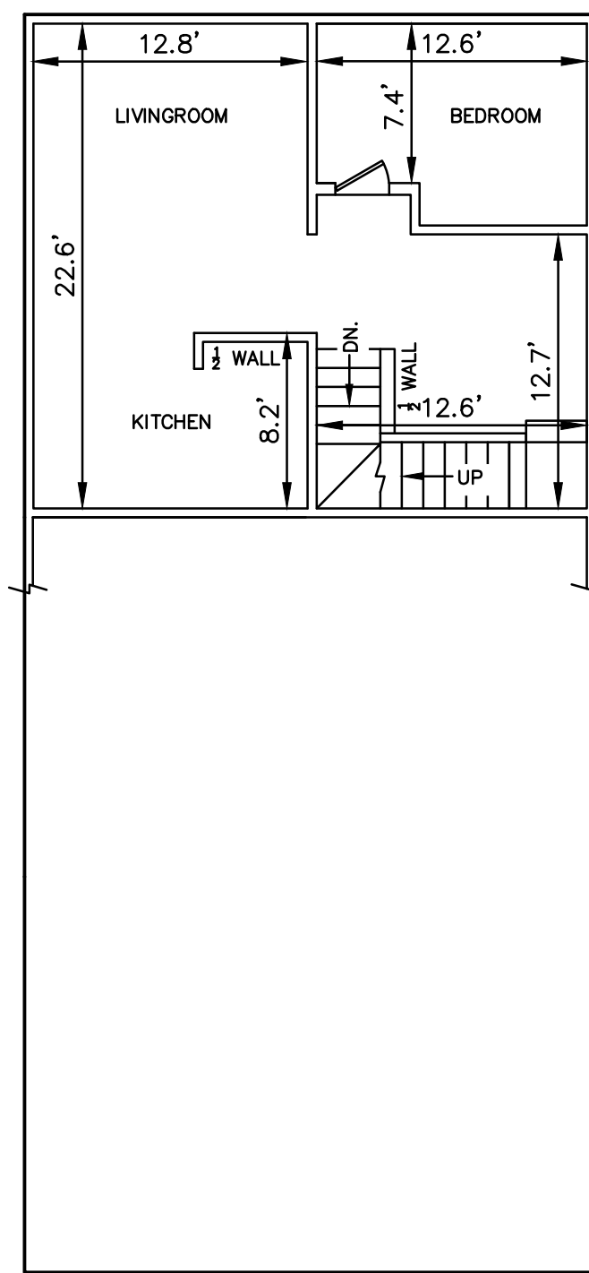
SECOND FLOOR UNIT #2 AREA=581.1 s.f.
