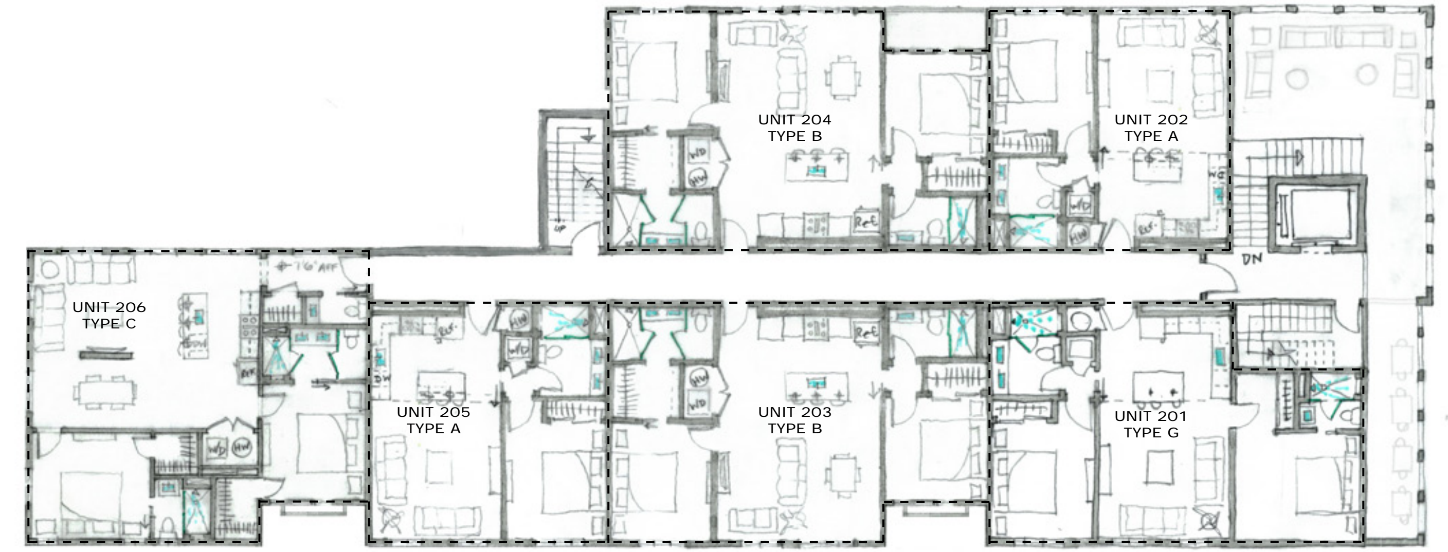
SECOND FLOOR PLAN SCALE 3/32"
