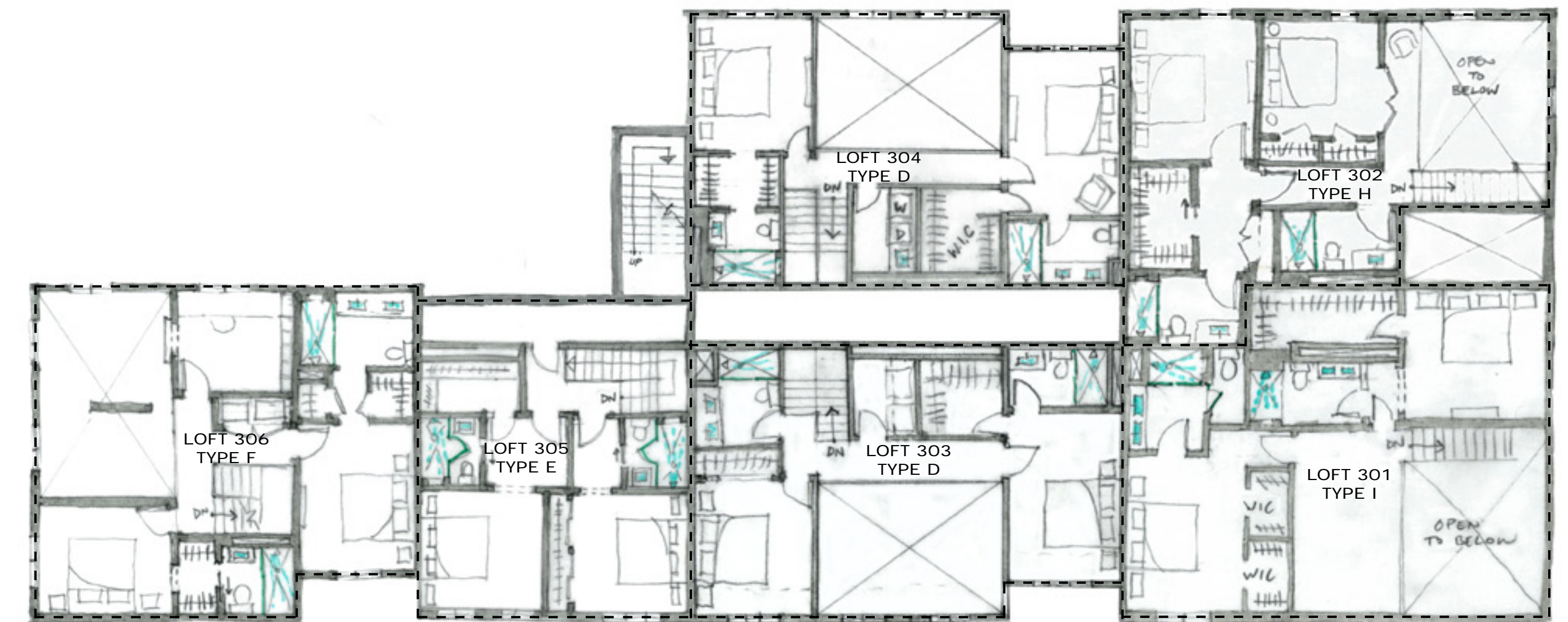
THIRD FLOOR LOFT SCALE 3/32"
