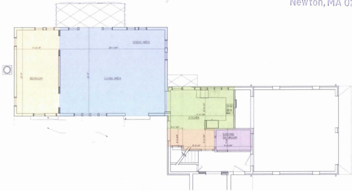
1 FIRST FLOOR PLAN - ACCESSORY APARTMENT
