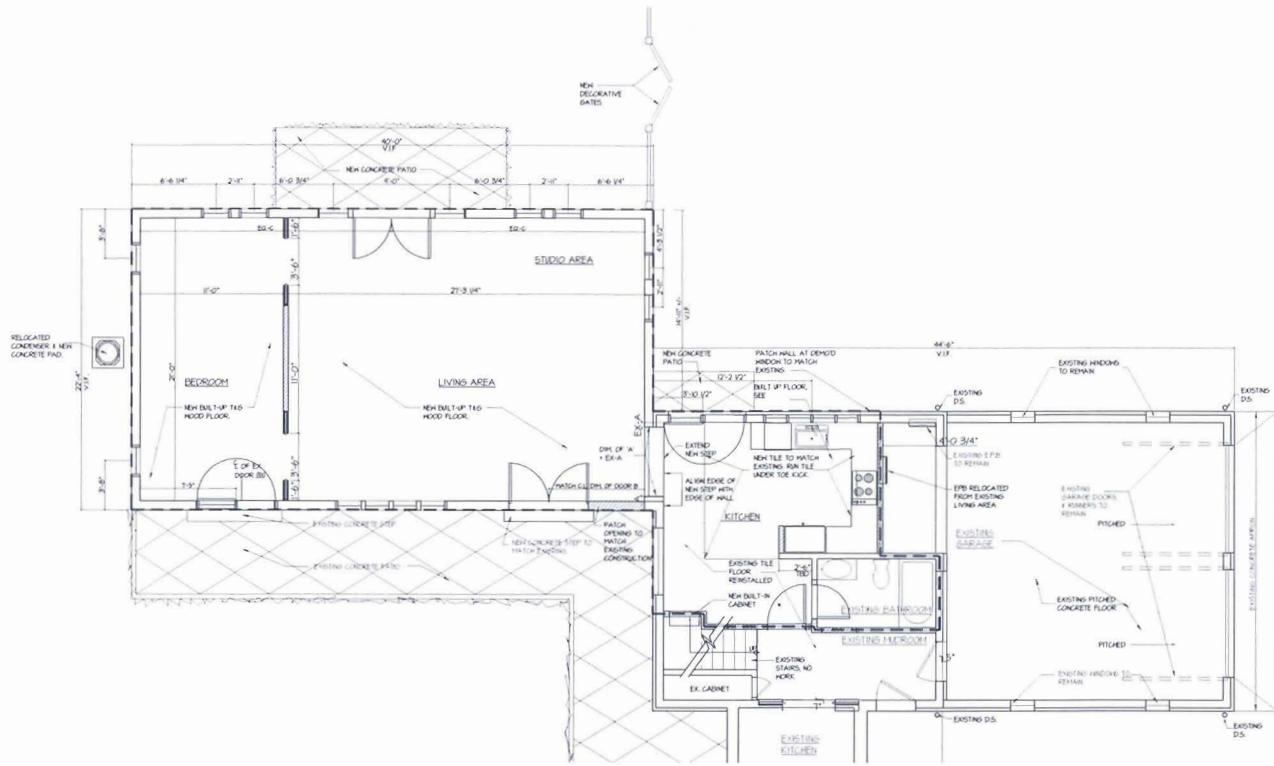
1 FIRST FLOOR PLAN - ACCESSORY APARTMENT
