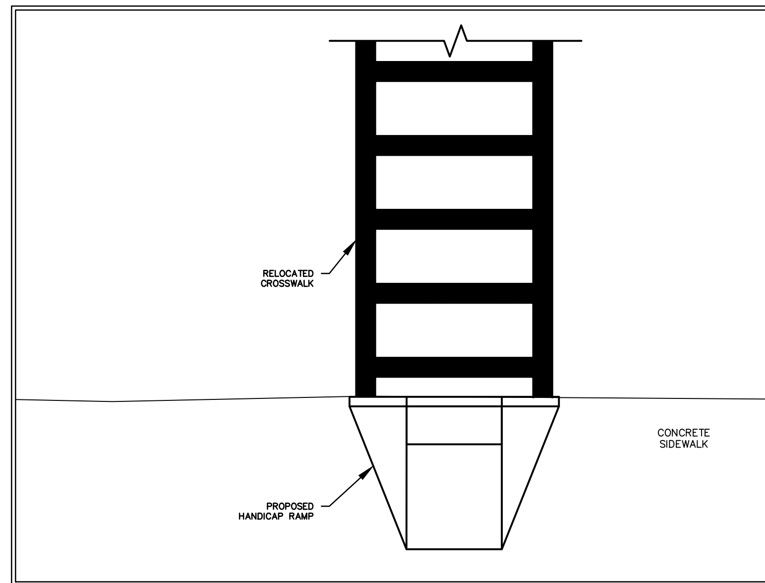
HANDICAP RAMP EXTENSION DETAIL NOT TO SCALE
