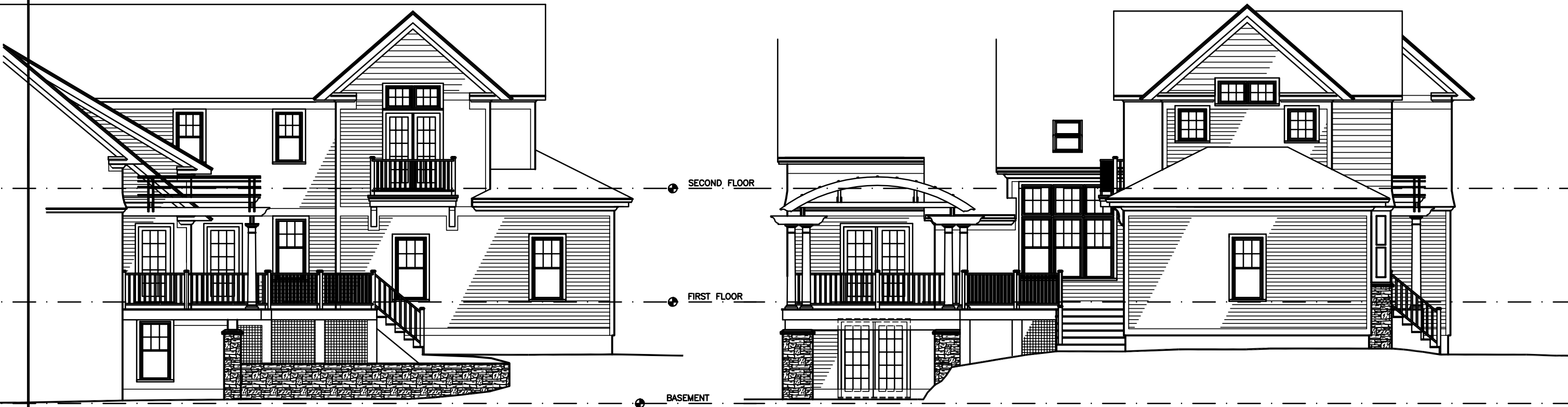
1 ELEVATION AT GARAGE REAR SIDE 1/4"=1'-0"
