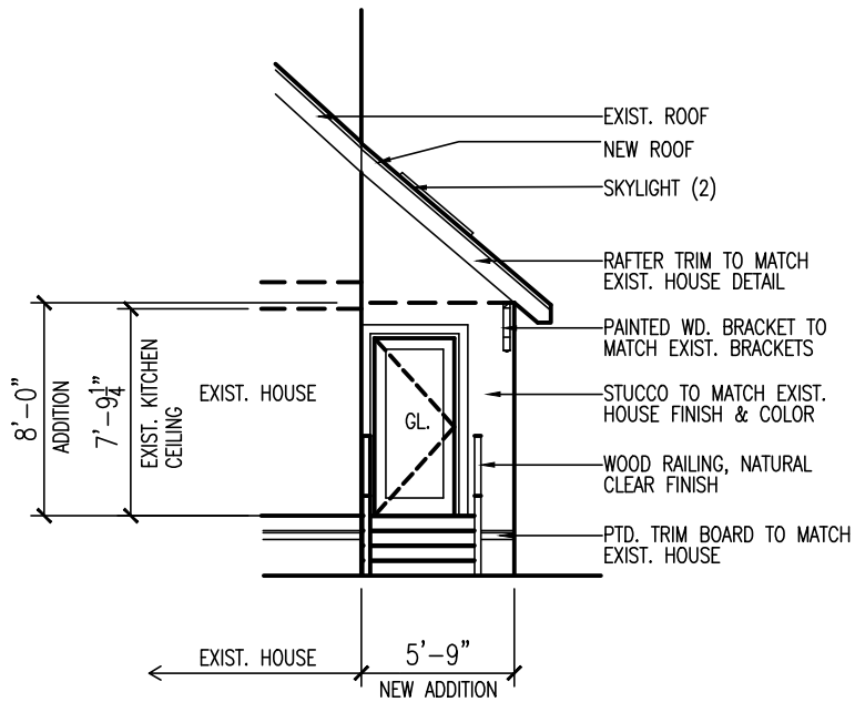
ENTRY TO MUDROOM ELEVATION
