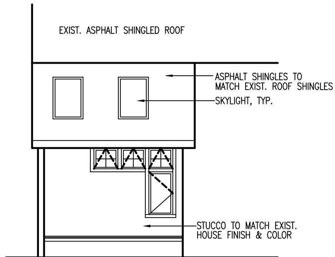
SIDE ELEVATION FACING NEIGHBOR
