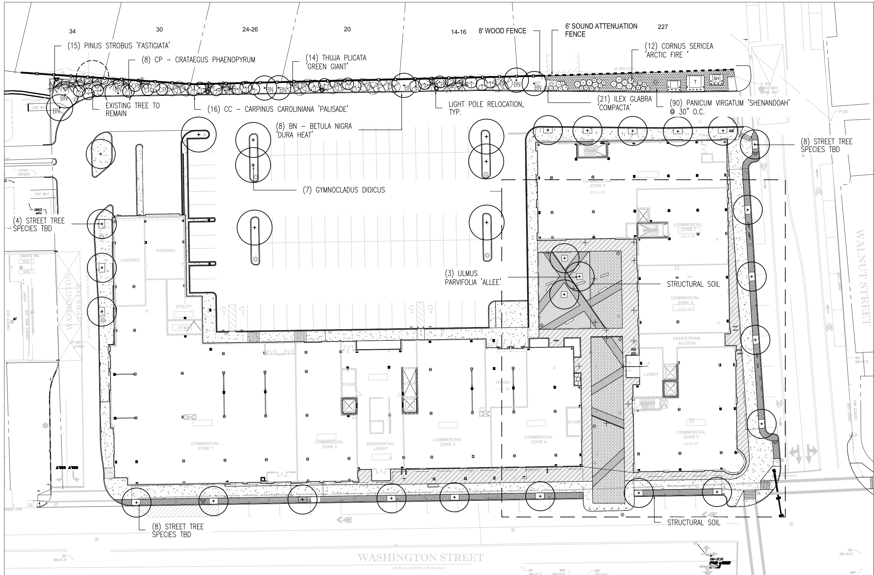
01 Landscape Plan SCALE: 1" = 40'-0"
