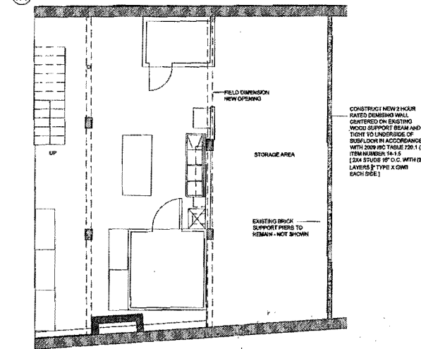
5 A-1 PROPOSED BASEMENT PLAN
