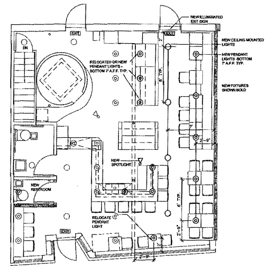
3 A-1 PROPOSED FIRST FLOOR CEILING & LIGHTING PLAN
