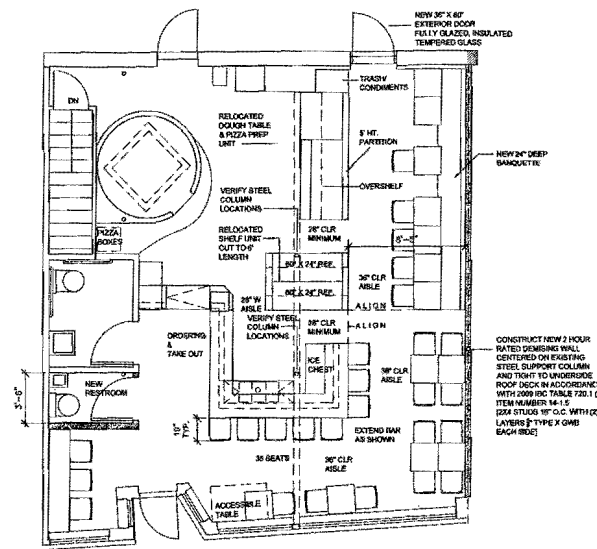
2 A-1 PROPOSED FIRST FLOOR PLAN
