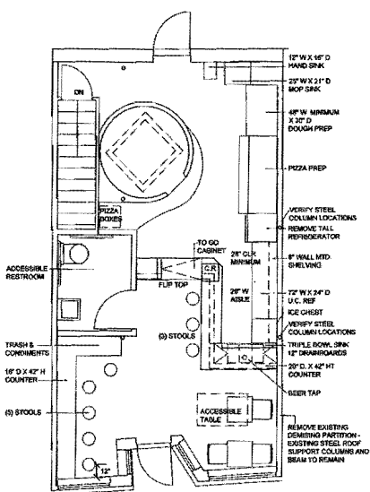
1 A-1 EXISTING FIRST FLOOR PLAN & DEMO
