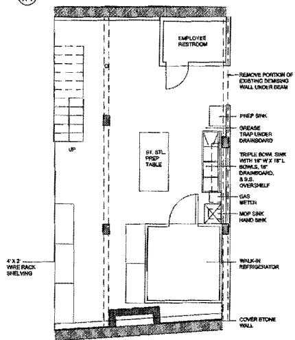
4 A-1 EXISTING BASEMENT PLAN & DEMO
