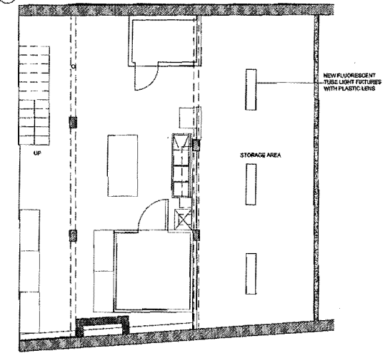
6 A-1 PROPOSED BASEMENT CEILING & LIGHTING PLAN
