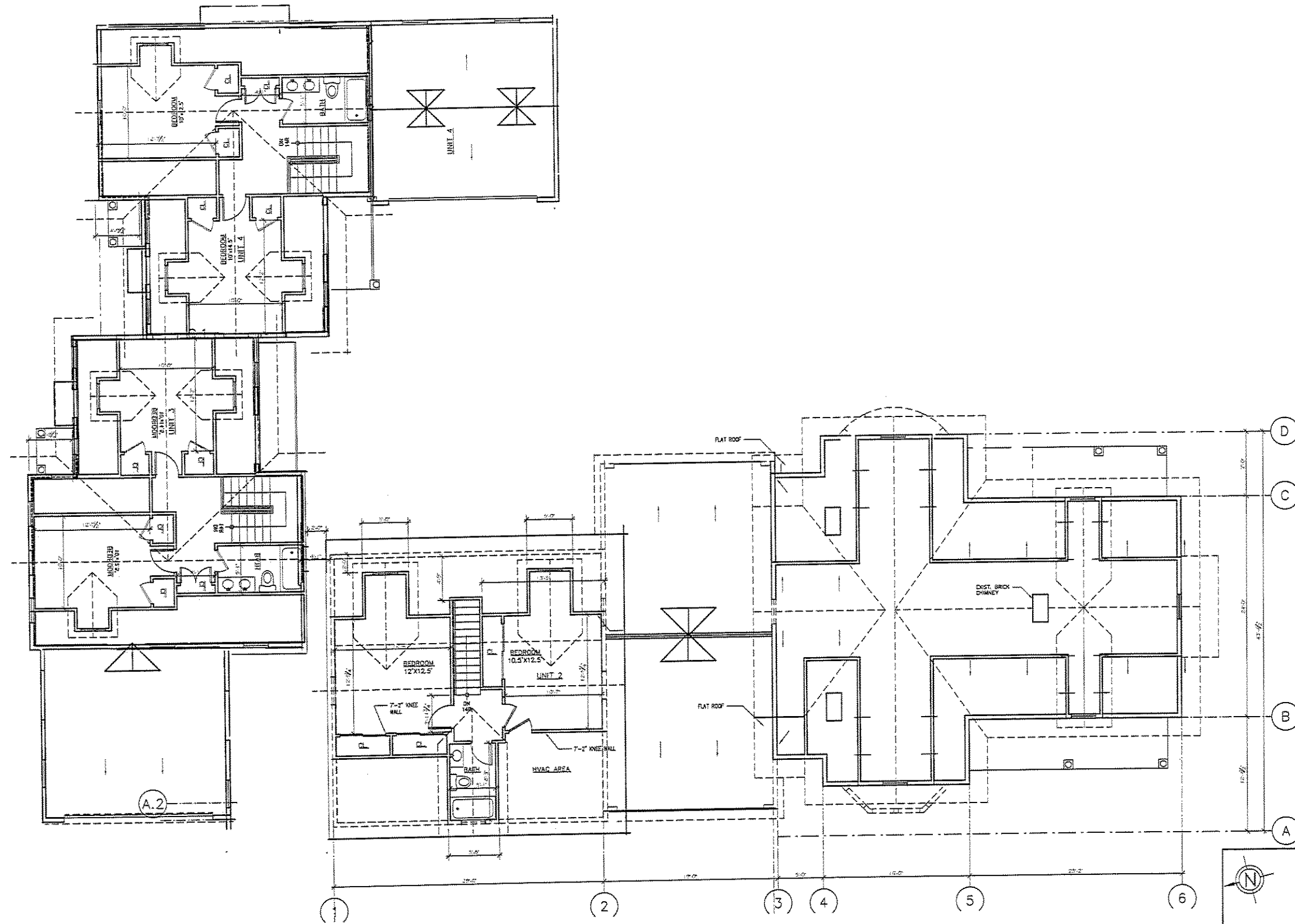
PROPOSED ATTIC FLOOR PLAN 1/4"=1'-0"
