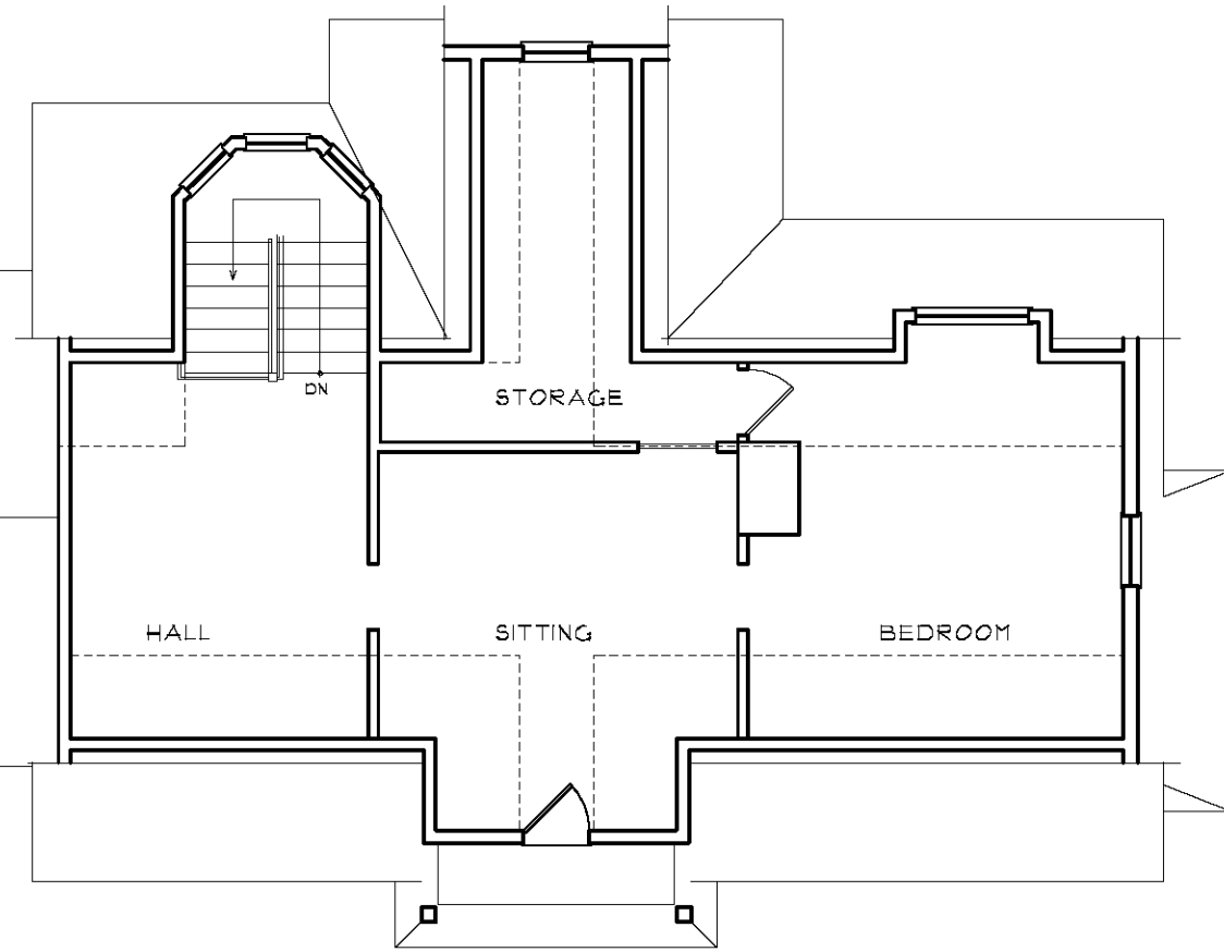
398 SF - Attic - Unit #1
