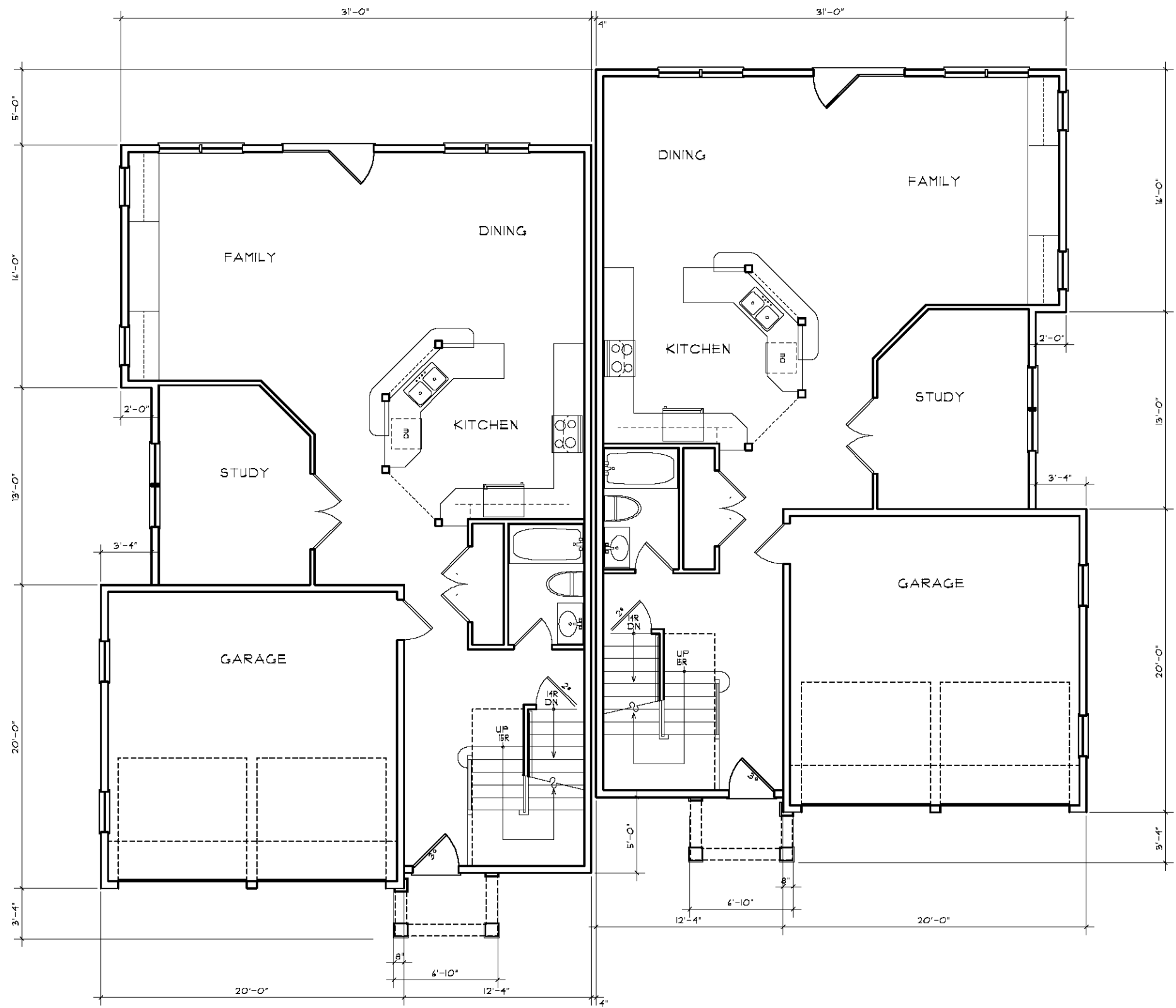
FLOOR PLANS - UNITS #3 & #4 1131 SF - Main Floor MAIN FLOOR PLAN
