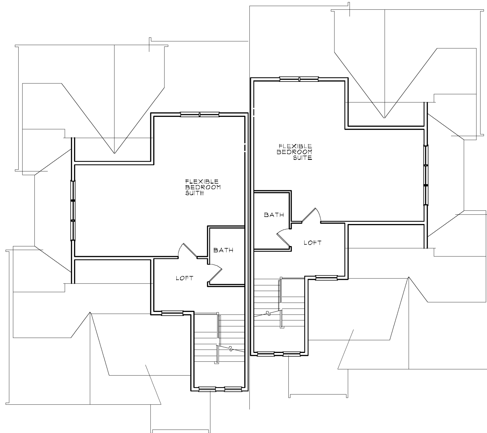
FLOOR PLANS - UNITS #3 & #4 554 SF - ATTIC ATTIC FLOOR PLAN
