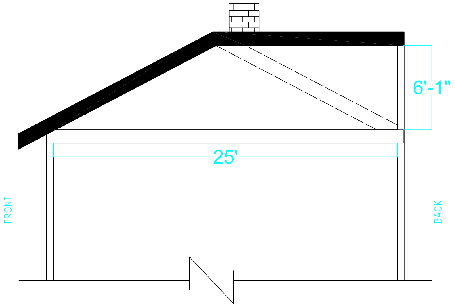
ARCHITECTURAL ELEVATIONS — SIDE VIEW
