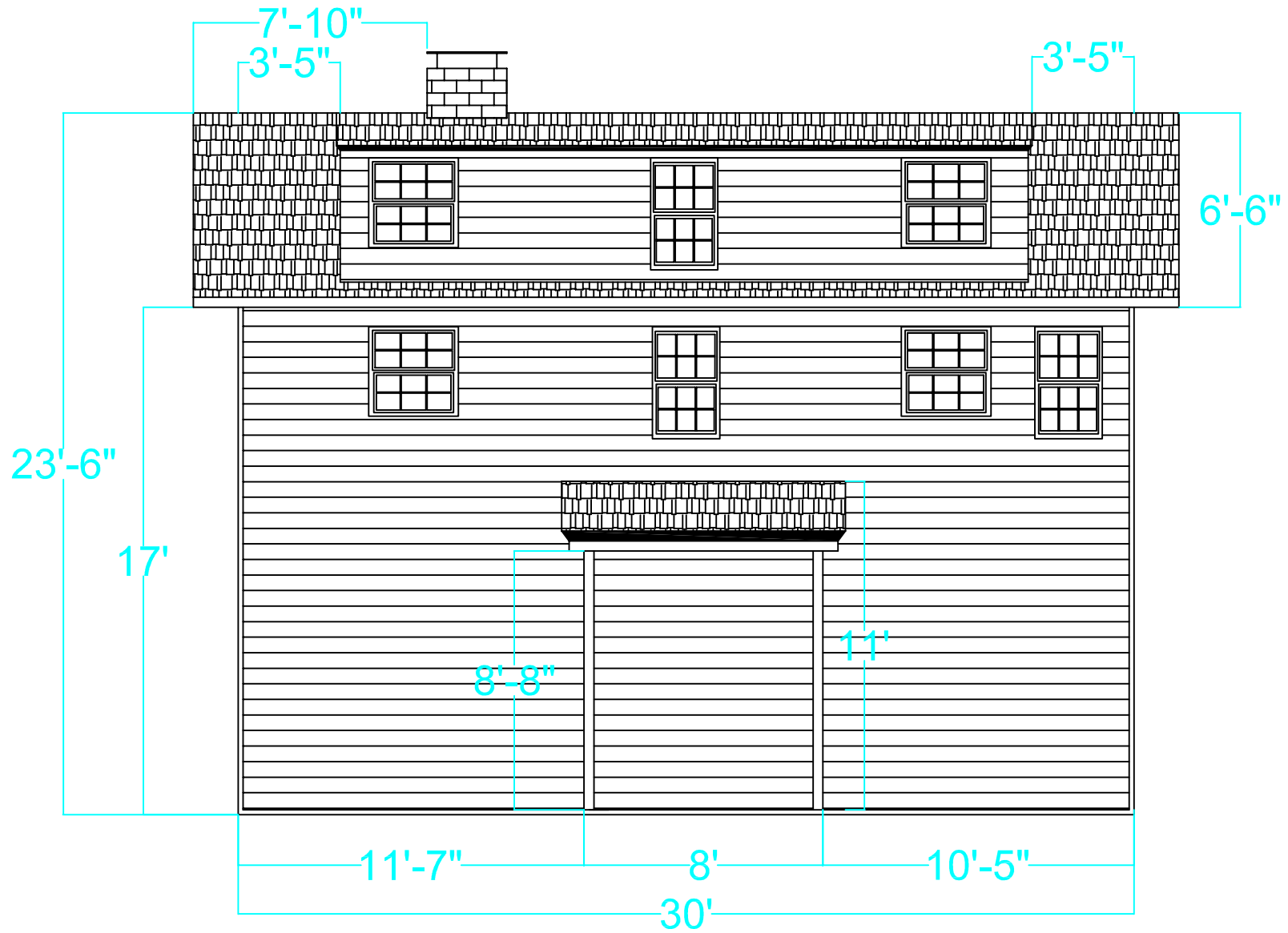
ARCHITECTURAL ELEVATIONS — REAR VIEW
