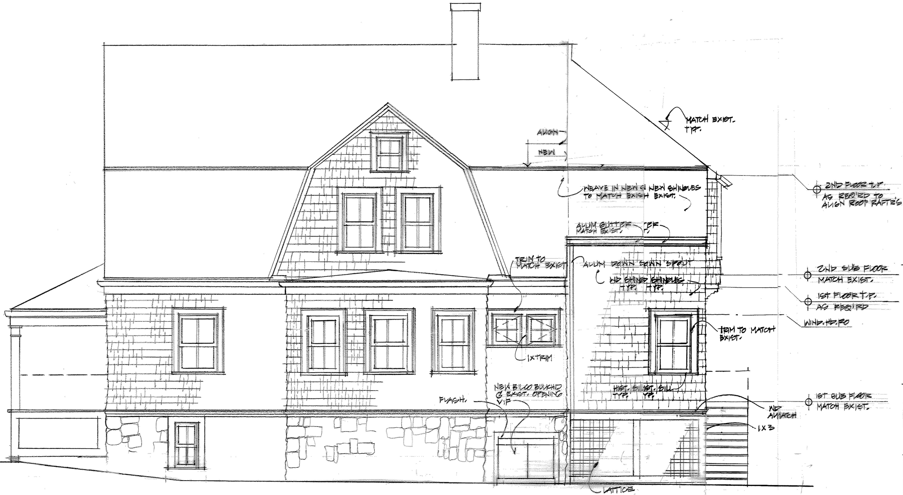
RIGHT ELEVATION 8/20/11
