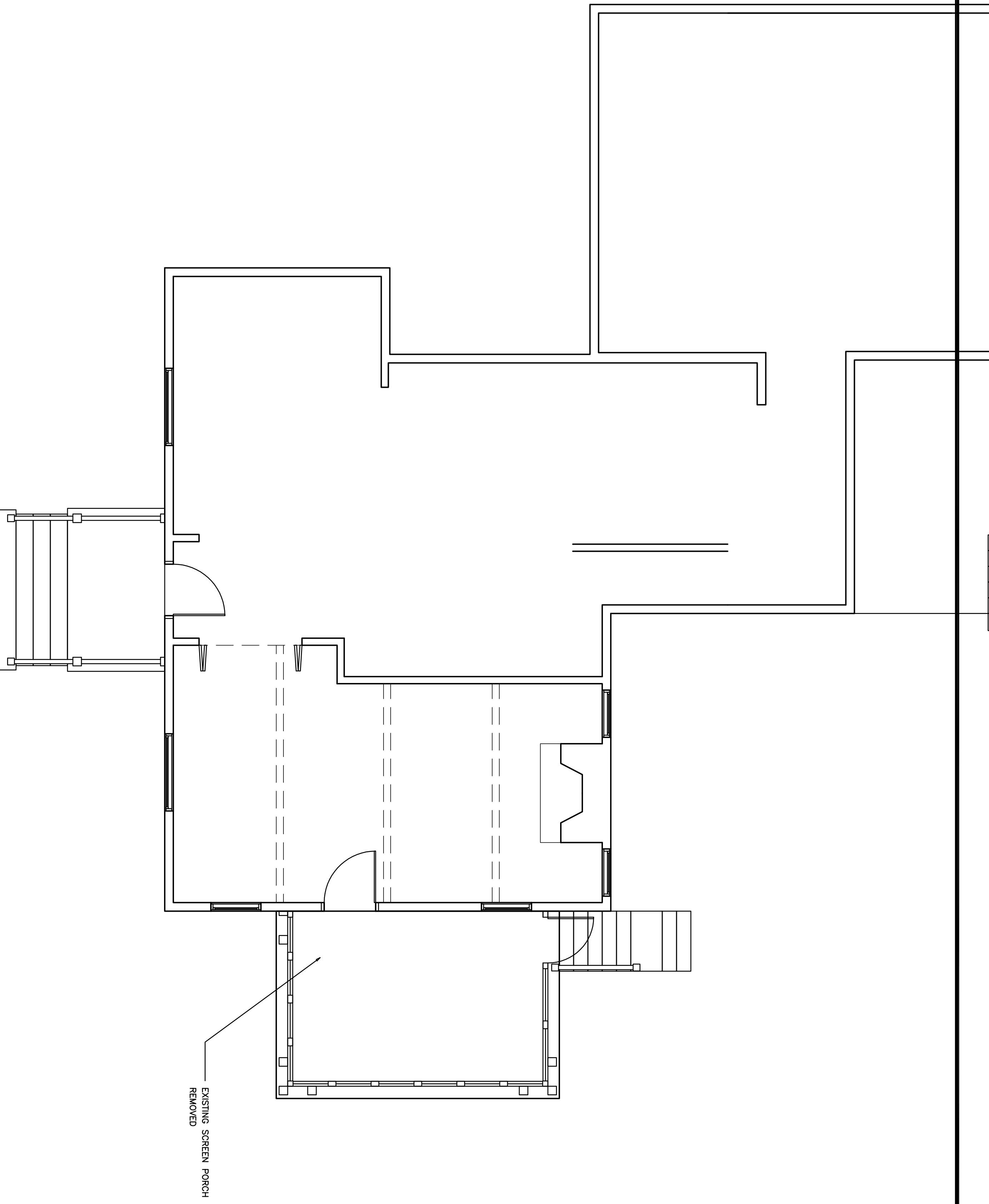
2 EXISTING PARTIAL FLOOR PLAN 1/4"=1'-0"
