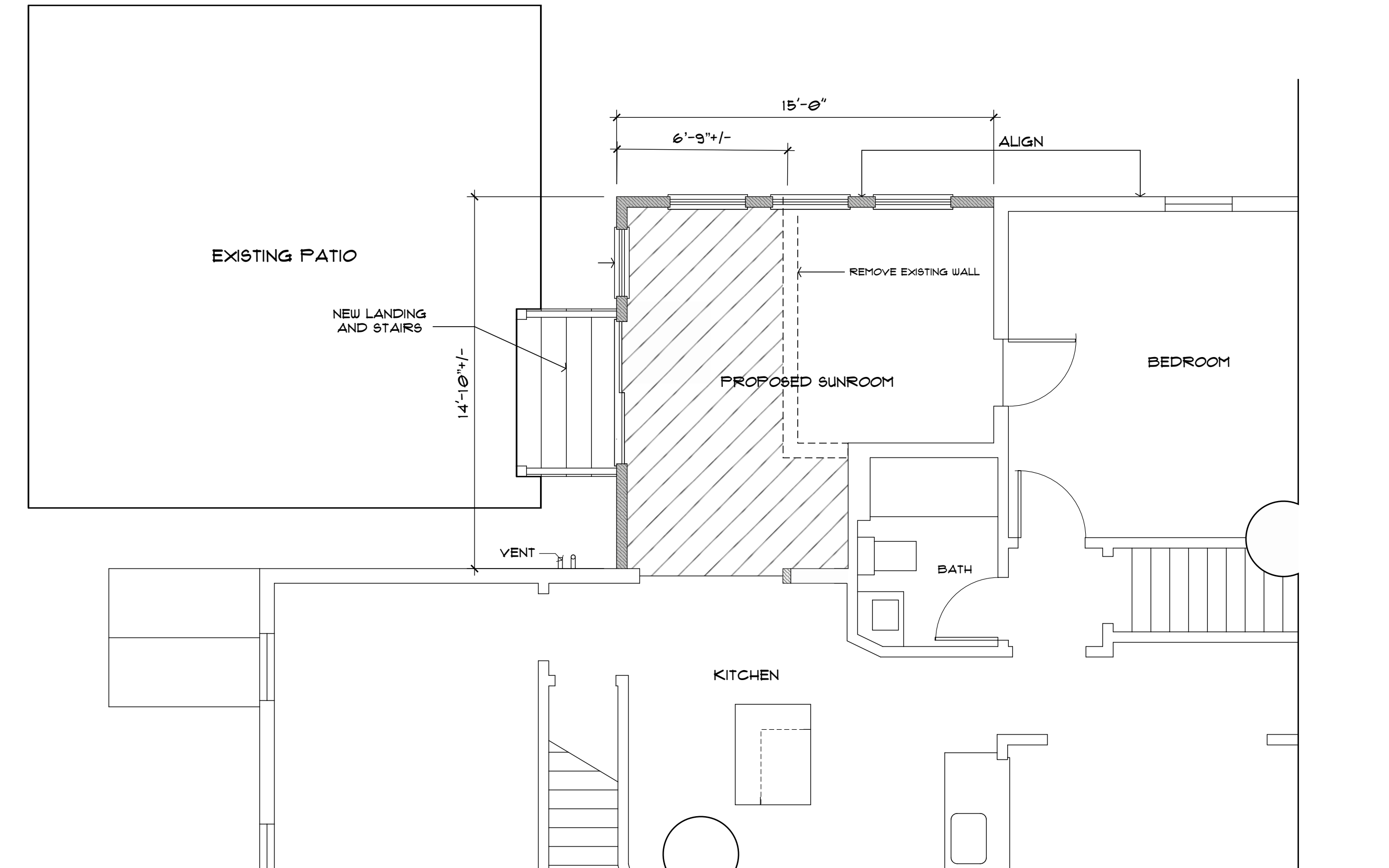
PROPOSED FLOOR PLAN 1/4"
