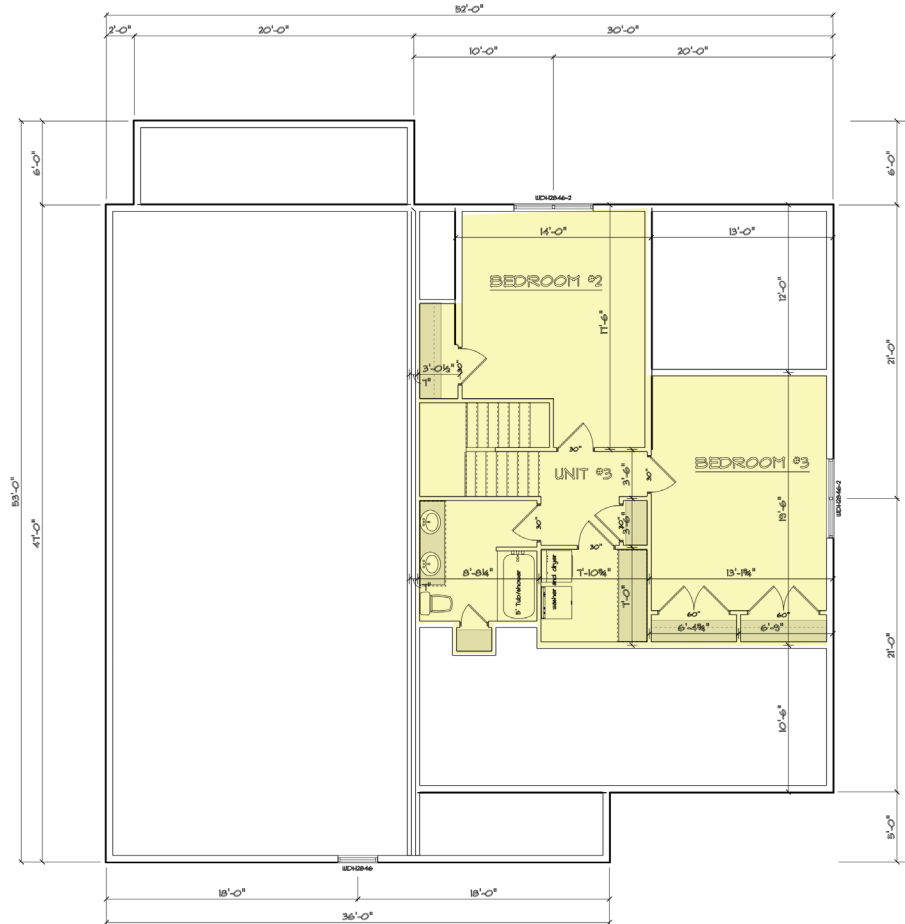
SECOND FLOOR PLAN 14'-11/2"
