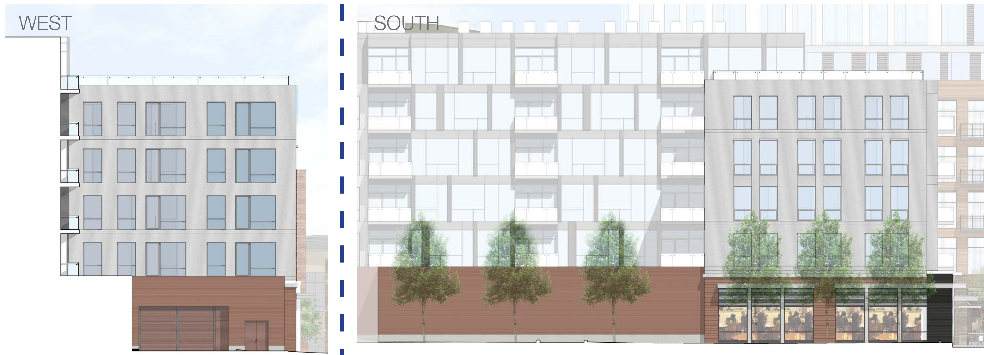
ELEVATED COURTYARD | SPECIAL PERMIT
