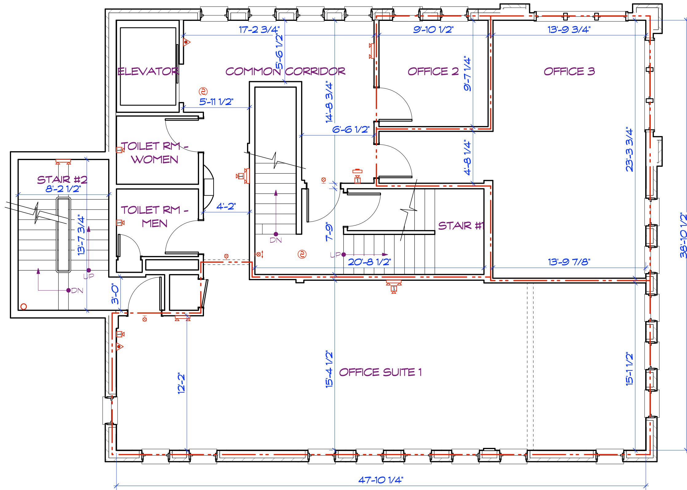
EXISTING SECOND FLOOR PLAN ② SCALE: 3/16" = 1'-0"
