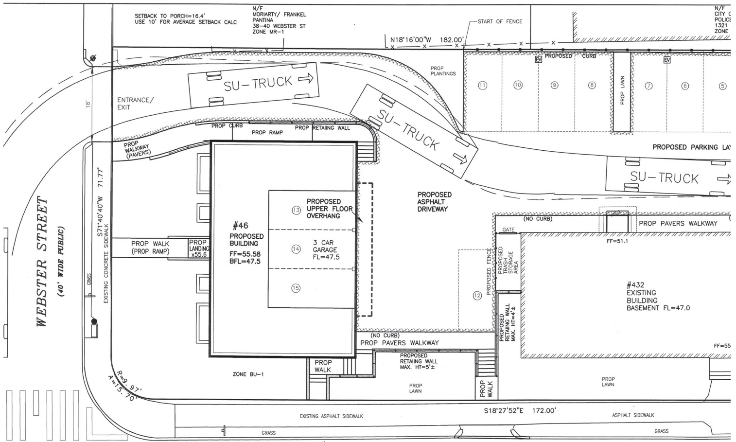
AASHTO SU-TRUCK ENTERING TURNING DETAIL SCALE: 1 IN. = 10 FT.
