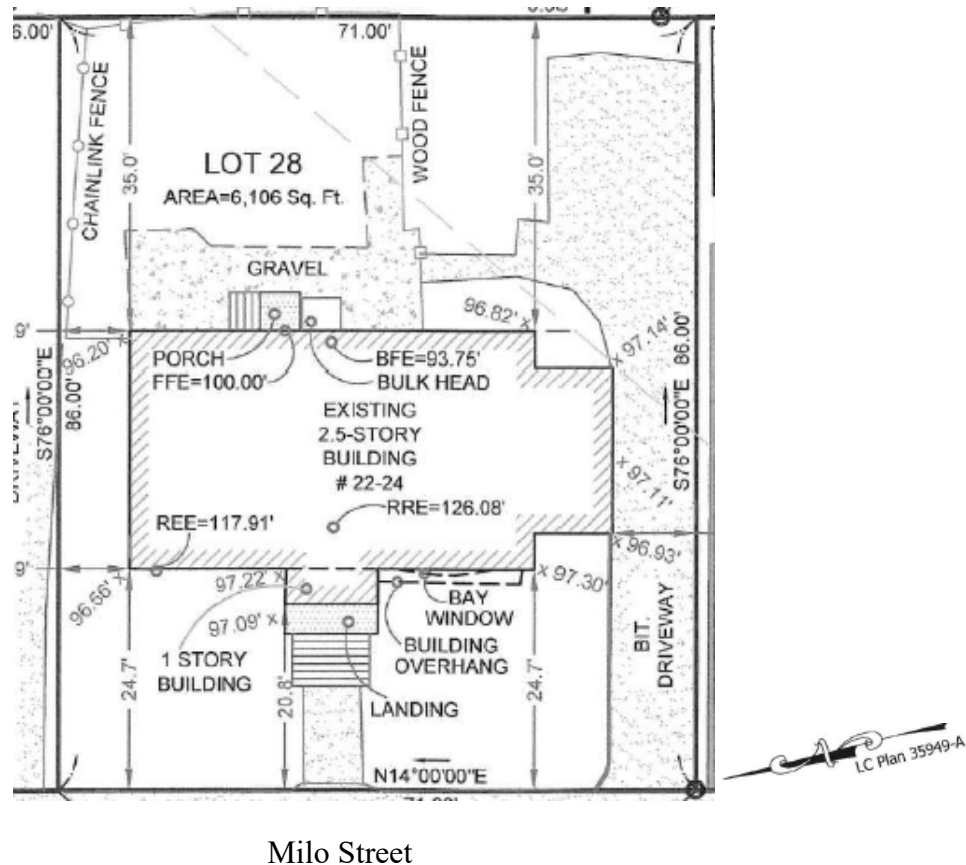
Existing Conditions Site Plan
