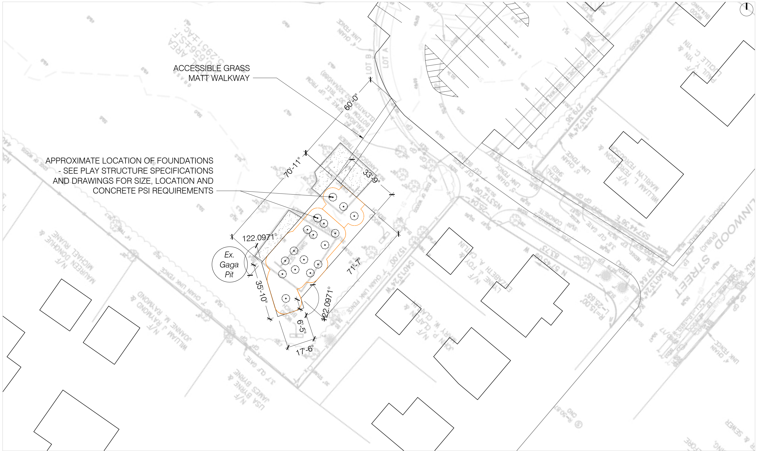
HORACE-MANN PLAYGROUND IMPROVEMENTS LAYOUT PLAN - EXHIBIT C
