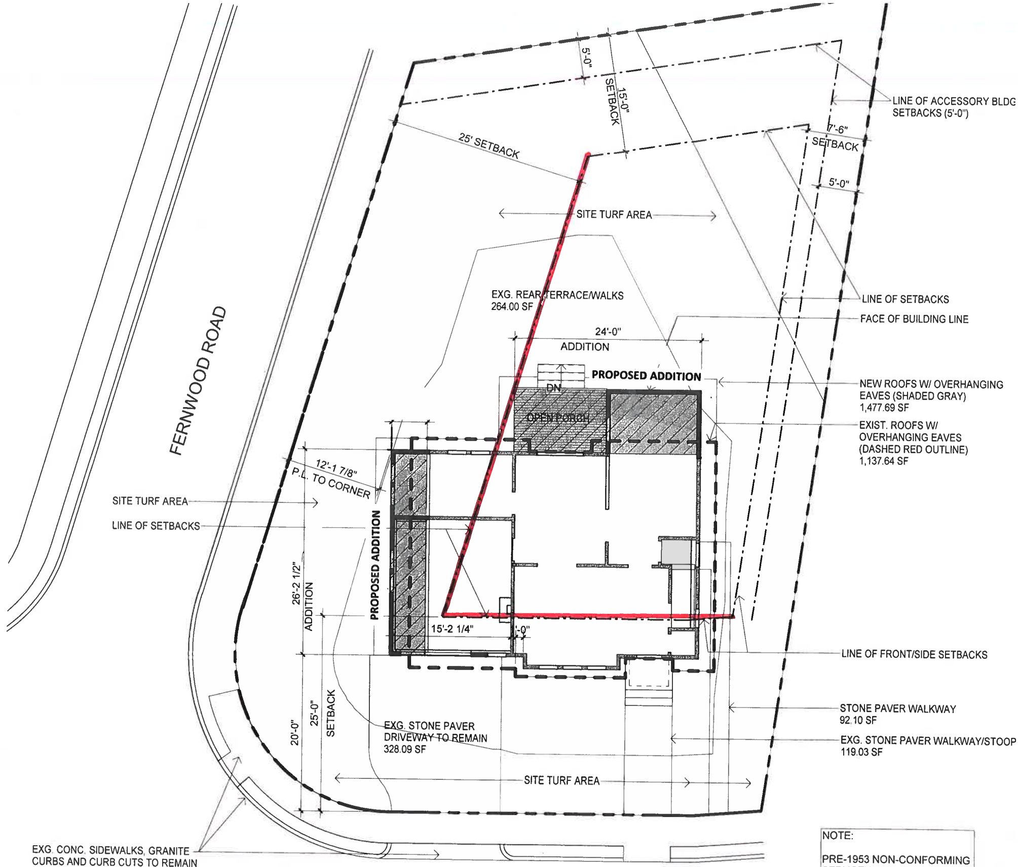
10 Proposed Site Plan A101 SCALE: 1" = 10'-0"
