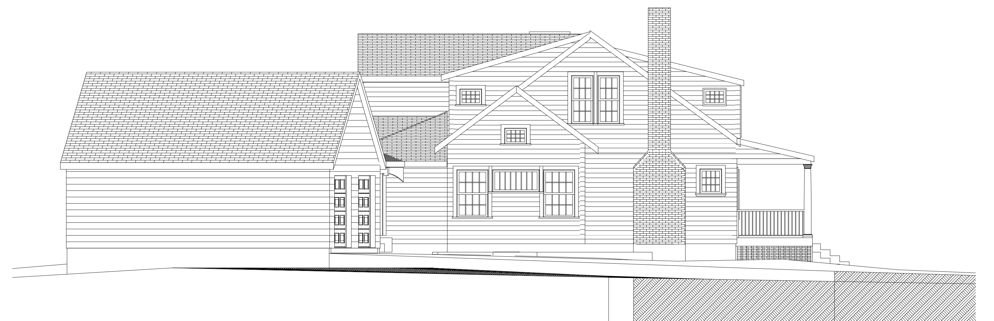
East Elevation-Proposed
