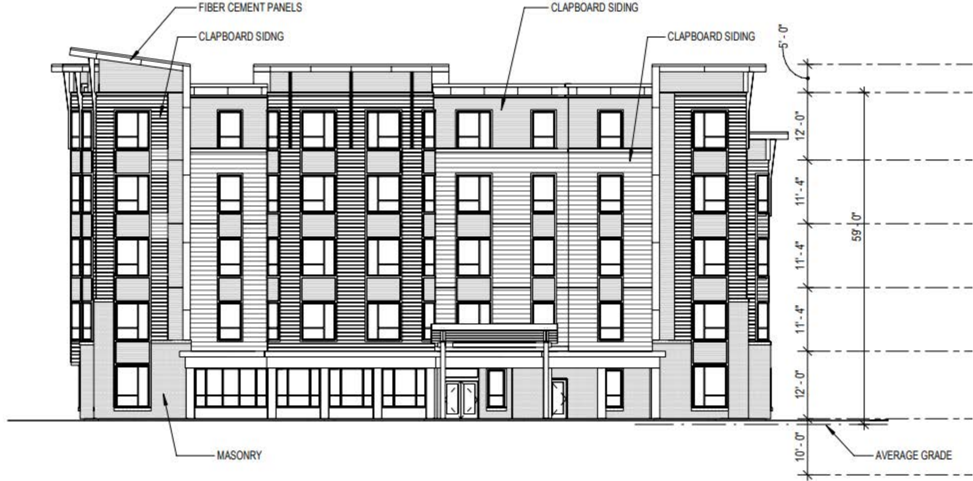
1 NORTH ELEVATION 1/16" = 1'-0"
