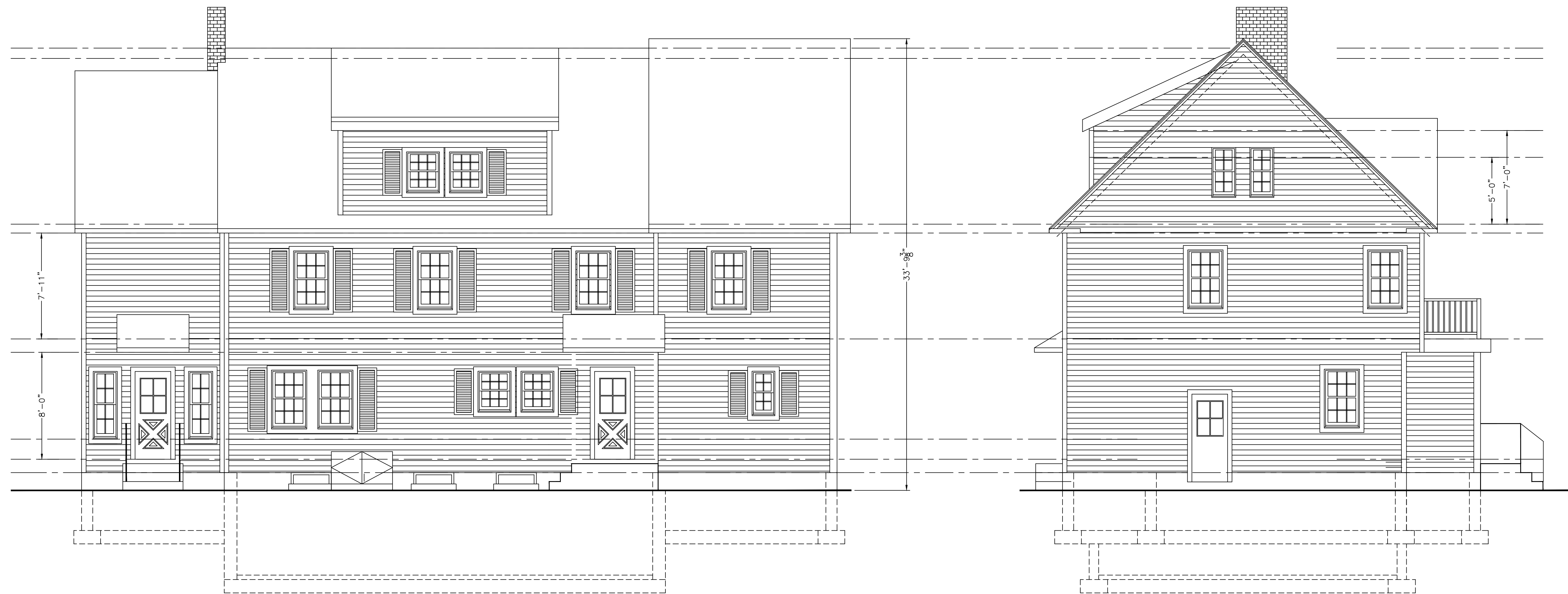
PROPOSED LEFT SIDE ELEVATION
