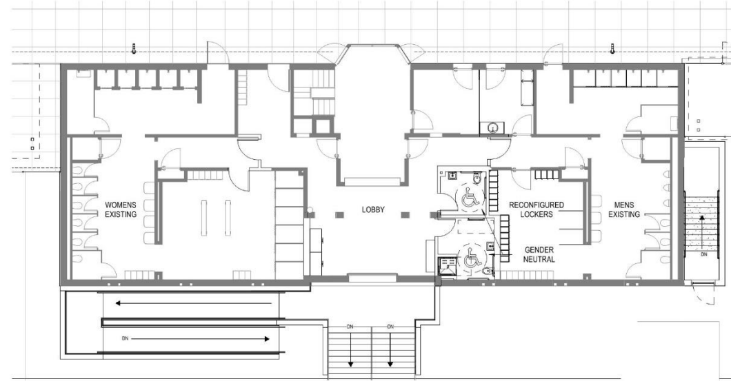
2 BATHHOUSE PLAN 1/8" = 1'-0"
